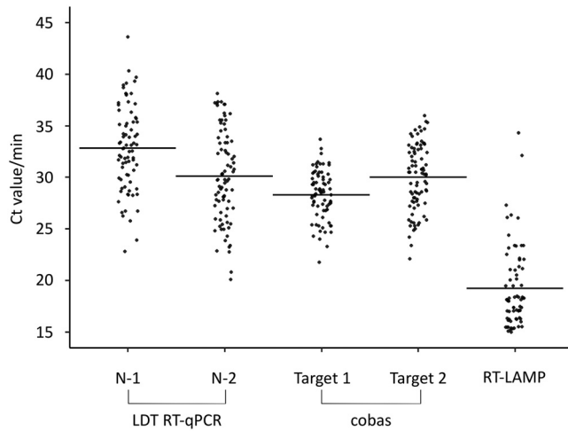
FIG 1 Cycle threshold ( C_T ) values and detection times for each molecular diagnostic test of saliva specimens. C_T value for each RT-qPCR primer set and detection time by reverse transcription–loop-mediated isothermal amplification (RT-LAMP). Horizontal lines indicate the mean C_T value or detection time.
