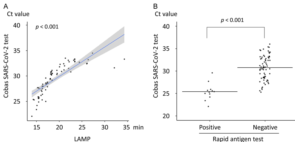
FIG 2 Relation of RT-qPCR, RT-LAMP, and the rapid antigen test (RAT) results for saliva specimens. (A) Relation between the detection time of reverse transcription–loop-mediated isothermal amplification (RT-LAMP) and the C_T value of target 2 (SARS-CoV-2 envelope gene) in the cobas SARS-CoV-2 test. The blue slope line represents the fitted regression curve. The gray shadow indicates the 95% confidence interval around the regression curve. (B) Distribution of the C_T values of target 2 for the cobas SARS-CoV-2 test of saliva with positive and negative results. Horizontal lines indicate the mean C_T value. The P value was calculated using Student’s t test.
