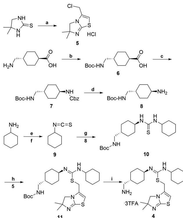
Scheme 2 Synthesis of aminomethyl-substituted IT1t (4). Reagents and conditions: (a) 4,4-dimethyl-imidazolidine-2-thione, 1,3-dichloroacetone, CH 3 CN, 1-methoxy-2-(2-methoxyethoxy)-ethane, 145 °C 50–60% (b) BOC 2 O, NaHCO 3 , 1,4-dioxane, –5 °C, 50–60% (c) DPPA, TEA, BnOH, 80 °C, 20–30% (d) Pd/C, MeOH, H 2 , 10 psi, rt, 90–95% (e) TEA, CS 2 , THF, 0 °C (f) TsCl, HCl, rt, 2 step 60–70% (g) CH 2 Cl 2 , 8, rt, 70–80% (h) CH 3 CN, reflux, 5, 50–60% (i) CH 2 Cl 2 , TFA, rt, 90–95%.
