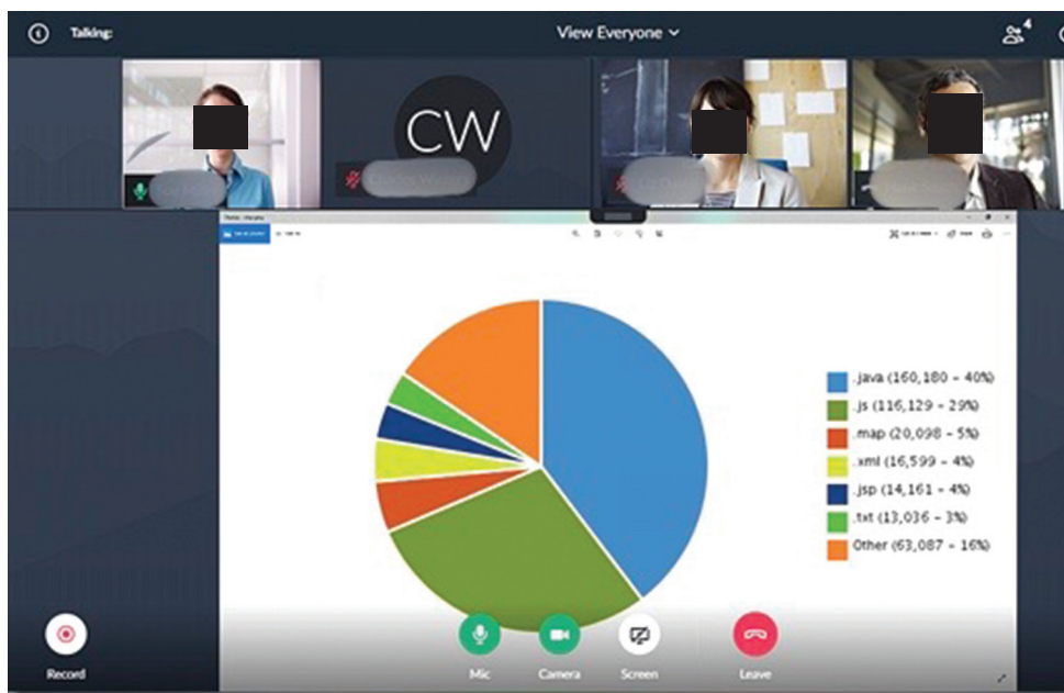
Fig. 2 GoToMeeting-meeting interface.
