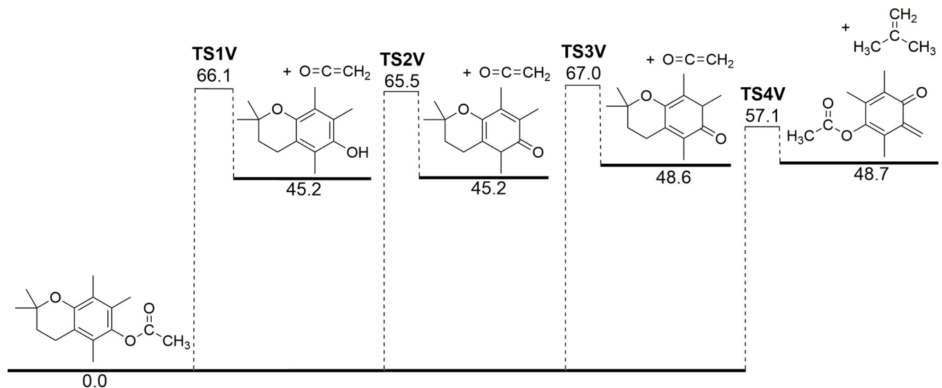
Fig 2. Potential energy diagram for the thermal decomposition of a vitamin E acetate model compound, VEA-MC. Energies (0 K enthalpies, kcal mol -1 ) are calculated at the DSD-PBEB95-D3(BJ)/def2-TZVPP level of theory.
