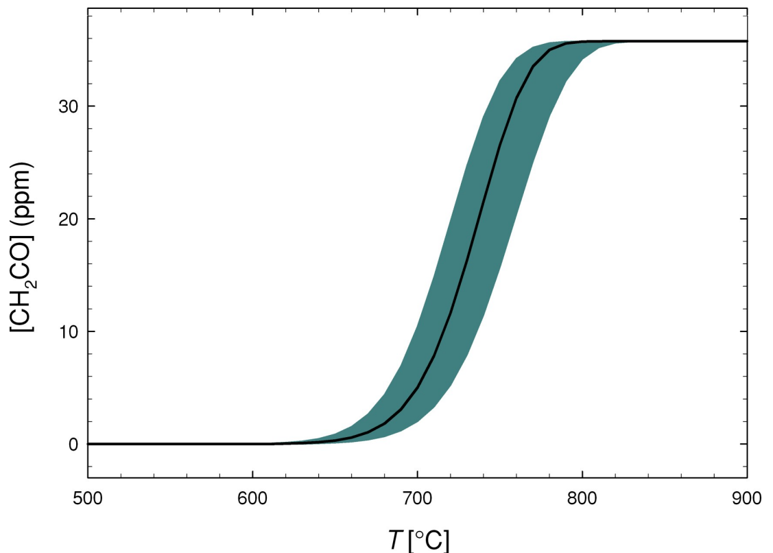
Fig 5. Predicted in-lung ketene concentration ( [\text{CH}_2\text{CO}] , ppm) from a single puff of vitamin E acetate contaminated e-liquid, as a function of temperature. Shaded area shows the uncertainty in predicted concentrations obtained by varying all activation energies by \pm 2 kcal/mol.
