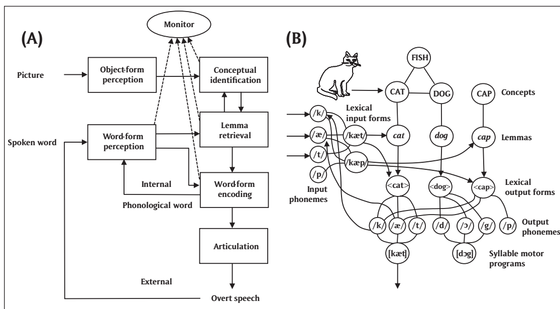
Figure 1: Illustration of comprehension-based self-monitoring in WEAVER++. (A) In naming a picture, the phonological word representation of the picture name is fed into the speech comprehension system (the internal loop), which also processes the overtly articulated picture name (the external loop). The monitor compares selected production and comprehension representations. (B) Network representing the word cat , whereby output phonemes activate input phonemes, which serves the internal monitoring loop.
