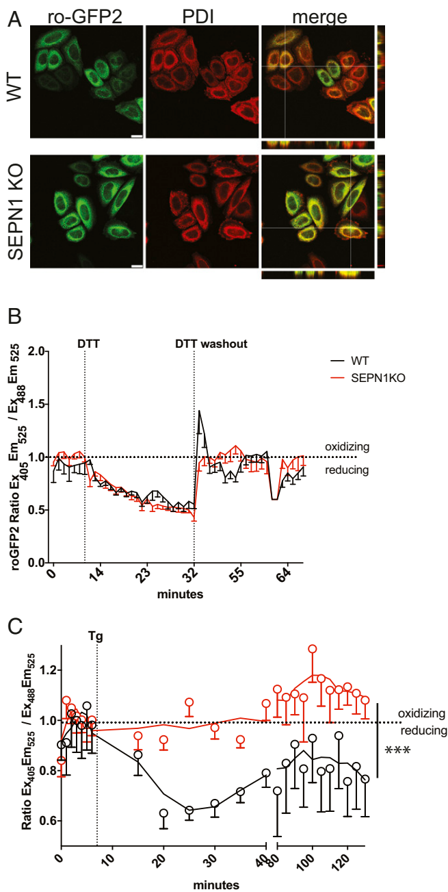
Fig. 6. A reducing shift is lacking in SEP1N KO cells after luminal calcium depletion. (A) Fluorescent photomicrographs of WT and SEP1N KO cells transiently expressing an ER-localized roGFP2, immunostained for PDI as an ER marker. The merged panels with orthogonal views show an overlap of the roGFP2 signal with PDI (Scale bar: 20 \mu m.) (B) Traces of time-dependent changes in the fluorescence excitation ratio of roGFP2, reflecting the alterations in the redox state of roGFP2 localized in the ER of WT and SEP1N KO cells. Cells were exposed to a DTT pulse of 20 min, followed by washout of the reductant. (C) Cells were exposed to the irreversible SERCA inhibitor Tg for 2 h. Each data point represents the mean \pm SEM of the fluorescence excitation ratio of roGFP2. The experiment was reproduced five times, with similar results ( P < 0.001 , two-way ANOVA) (SI Appendix, Fig. S5B).
