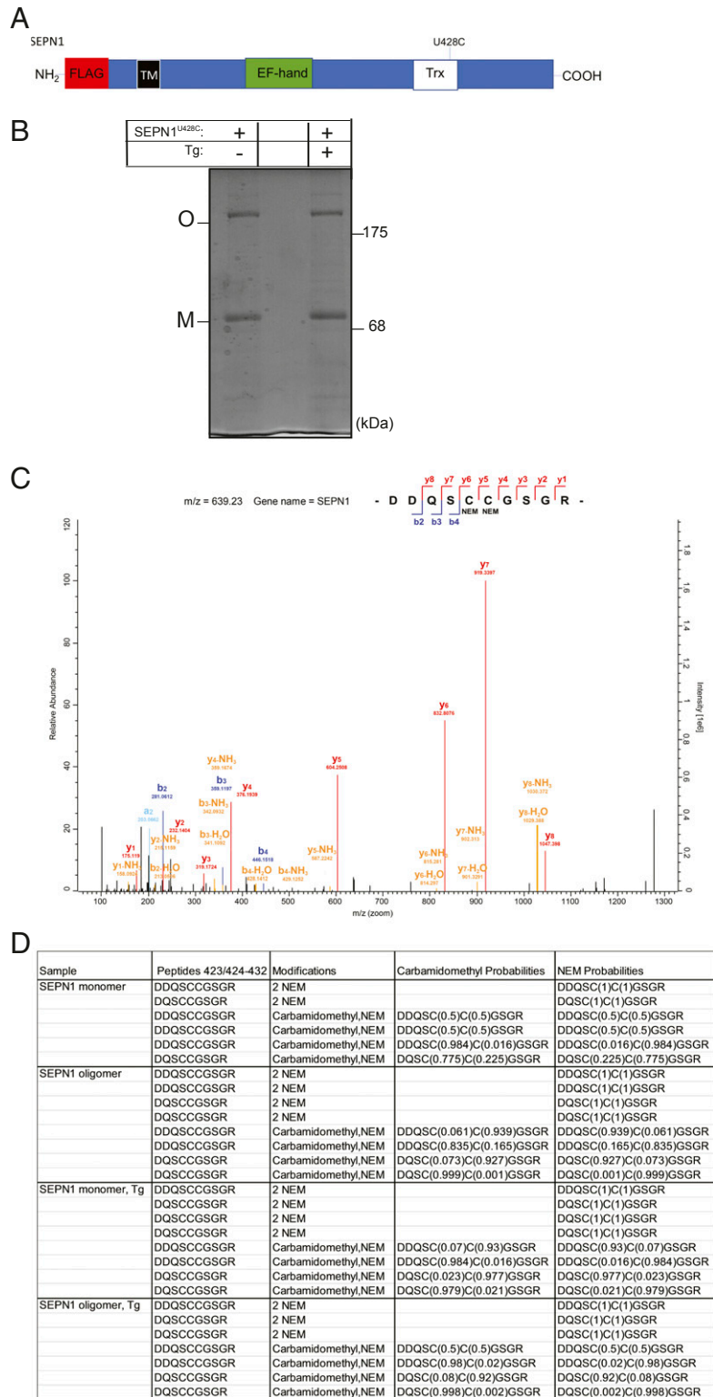
Fig. 4. The attacking amino acid of SEPN1 in Trx domain is present in a reduced form. (A) Schematic representation of a SEPN1 construct exploited in the experiments related to this figure. (B) Coomassie blue-stained nonreducing SDS/PAGE of FLAG-immunopurified SEPN1 after treatment with Tg or DMSO indicating the bands of the monomeric (M) and oligomeric (O) form that were cut and the redox state of cysteines analyzed by nLC-ESI-MS/MS sequence analysis. Lane 1, transfected SEPN1 U428C and treated with DMSO; lane 2, empty; lane 3, transfected with SEPN1 U428C and treated with Tg. (C) Representative MS/MS spectrum for the peptide (423 to 432) derived from the monomer of SEPN1 and bearing NEM-alkylation of cysteines 427 and 428. (D) The redox state of cysteines 427 and 428 in SEPN1 after treatment with Tg or DMSO. Alkylation is reported as +NEM if the cysteines are alkylated by NEM and present in a reduced form or as +carbamidomethyl if the cysteines are alkylated by IAA and present in an oxidized form. The probability of different alkylation types (derived from MaxQuant analysis) is reported in parentheses.
