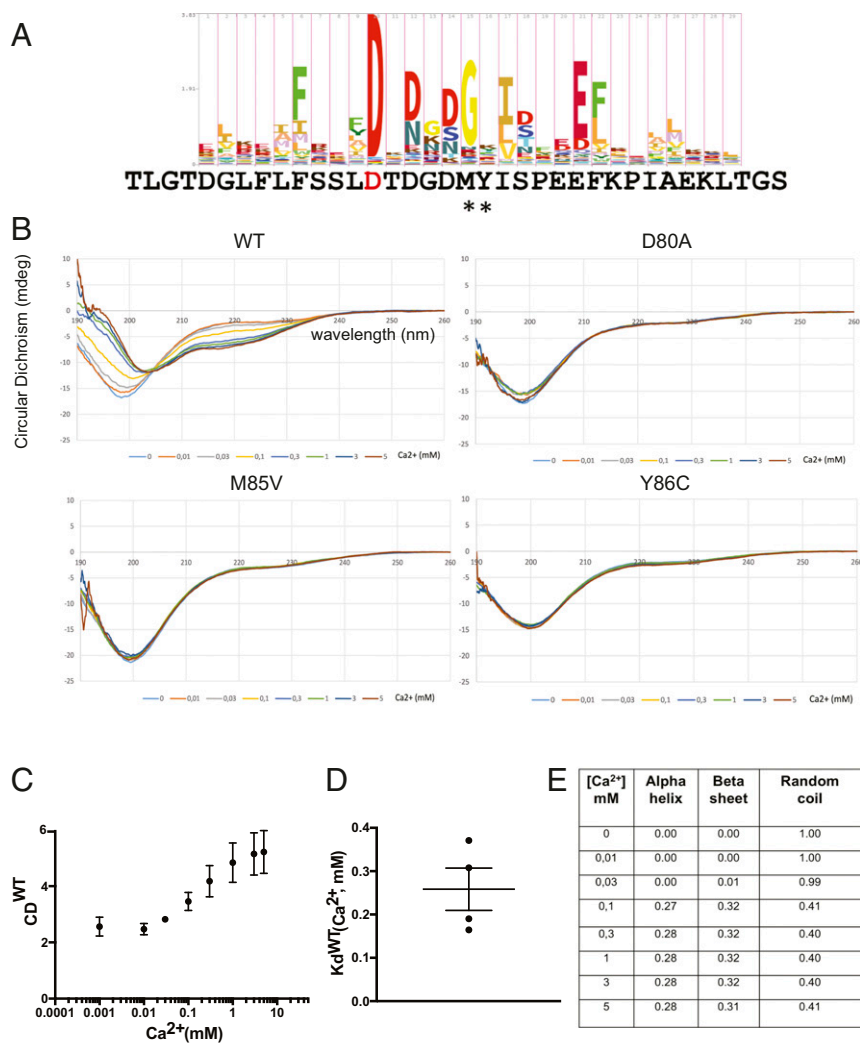
Fig. 2. Ca 2+ binding and Ca 2+ -dependent conformational change in SEPNI. (A) Alignment of SEPNI predicted EF-hand sequence to the EF-hand HMM logo plot (obtained from PFAM; https://pfam.xfam.org/family/PF00036#tabview=tab4 ). The important conserved amino acid D80 within the SEPNI sequence, depicted in red, was mutated to A. Pathogenic mutants identified within this sequence are highlighted by a star and correspond to the mutants M85V and Y86C. Residue numbering is based on UniProt entry Q9NZV5. (B) CD spectra of the indicated peptides at different calcium concentrations (0 to 5 mM). (C) CD (mdeg) values at 220 nm of the WT peptide at different calcium concentrations. (D) K d Ca 2+ of WT calculated from CD values at 220 nm in four different experiments with different peptide preparations. (E) Analysis of the secondary structure of the WT by the K2D algorithm ( dichroweb.cryst.bbk.ac.uk/ ).
