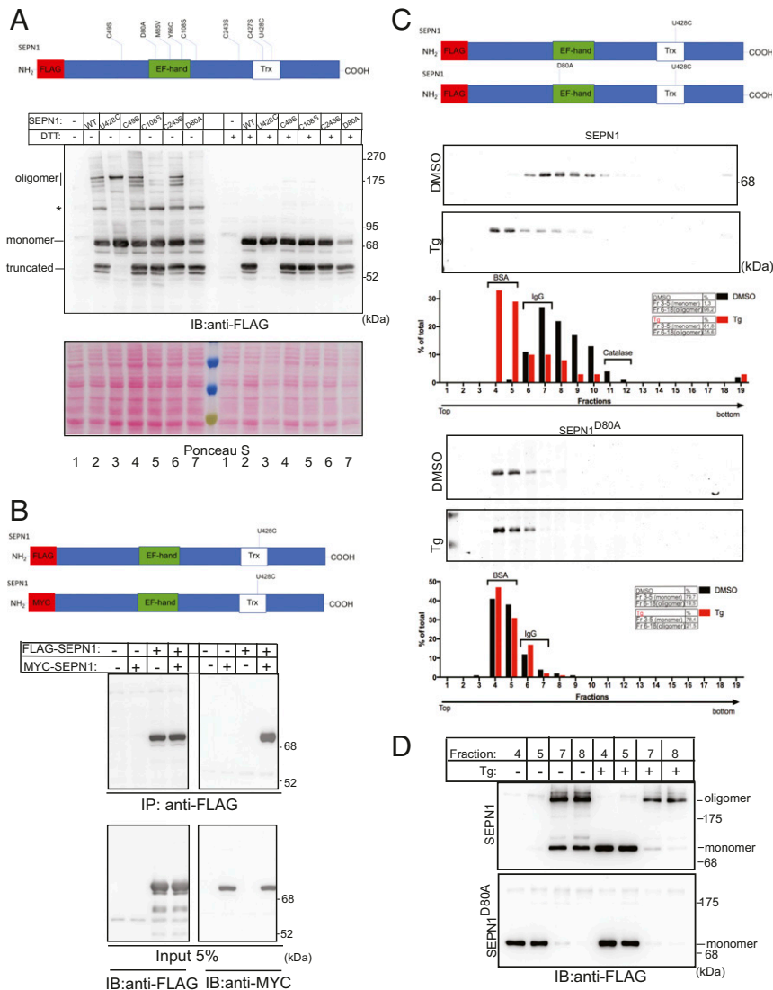
Fig. 3. Ca 2+ -dependent oligomeric change of SEPN1 in cells. (A) Scheme of FLAG-SEPN1 protein and its mutants. The EF-hand domain, the Trx domain, and all the amino acid mutants are noted. Below are nonreducing and reducing FLAG immunoblots of the indicated FLAG-SEPN1 and its mutants. The truncated, monomeric, and oligomeric SEPN1 are indicated. The asterisk indicates an additional band that is visible for the selenocysteine-containing form and whose origin was not analyzed. Membrane staining with Ponceau S is shown as protein-loading control. (B) Scheme of FLAG-SEPN1 and MYC-SEPN1 protein. Immunoblot of MYC-tagged SEPN1 immunoprecipitated with FLAG-M2 antibody from lysate of HeLa cells that were untransfected or transfected with expression plasmids of the indicated proteins. The lower two panels represent 5% of the total input protein lysate immunoprecipitated. The proteins were resolved on reducing SDS/PAGE. (C) Sucrose gradient analysis of FLAG-SEPN1 and FLAG-SEPN1 D80A in HeLa cells treated for 2 h with DMSO or Tg. Samples were analyzed on 4% to 20% sucrose gradients. Equal aliquots of the 19 fractions were analyzed by FLAG immunoblotting. The positions and the molecular weight of size markers (BSA, IgG, and catalase) are established from Coomassie blue-stained gel. The tables on the right indicate the percentages of the monomer and the oligomer. (D) Nonreducing FLAG immunoblotting of the peak fractions of BSA (of similar size as the SEPN1 monomer) and IgG (of similar size as the oligomer) indicating that SEPN1 protomers are kept together to form the oligomer not only by a disulfide bridge (running as an oligomer), but also by weak interactions (running as a monomer).
