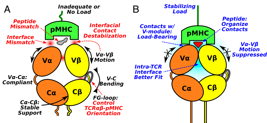
Fig. 6. Proposed mechanism of antigen screening and catch bond activation in \text{TCR}\alpha\beta -pMHC. (A) Mismatching interfaces, the \text{V}\alpha - \text{V}\beta motion, and orientation of the V-module relative to the C-module destabilize contacts with pMHC. Due to the dynamic nature of the contacts with pMHC, without a proper load, the complex is not sufficiently stable even with the agonist pMHC. (B) With a matching pMHC under a loaded state, the \text{V}\alpha - \text{V}\beta motion is suppressed through the load-bearing contacts with MHC. Deformation of \text{TCR}\alpha\beta also enhances overall fit among the various interfaces. The antigenic peptide plays a more significant role in organizing the interfacial contacts rather than bearing the load.
