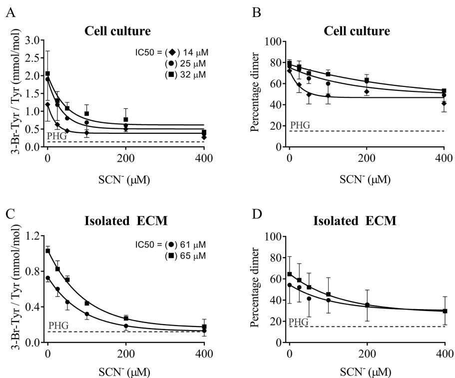
Figure 7. Effects of thiocyanate on the formation of 3-Br-Tyr and sulfimine crosslinks. A, 3-Br-Tyr and B, NCD dimer in PFHR9 cells cultured for 6–8 days in the presence of varying concentrations of SCN - either without added Br - (filled black diamond) or with 50 μM (filled black circle) or 100 μM Br - (filled black square) added. C, 3-Br-Tyr and D, NCD dimers, ECM isolated from PFHR9 cells cultured in the presence of PHG was treated with 50 μM H 2 O 2 and 50 μM (filled black circle) or 100 μM (filled black square) Br - , plus the indicated concentrations of SCN - for 1 h at 37°C. 3-Br-Tyr and dimer analyses were performed as described in Figs. 1 and 2. Values represent the means of three independent biological repeats ± S.D. The gray dashed lines represent inhibition by 50 μM PHG. IC 50 values were calculated from exponential decay curves in each figure. Error bars are shown in one direction for clarity and are not visible when they are within the symbol size. Curves represent nonlinear regression lines selected to give best fit to the experimental data points.
