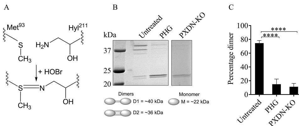
Figure 1. Formation of the sulfilimine crosslinks in the ECM during cell growth in culture. A, the structure of the sulfilimine bond between Met 93 and HyI 211 at the NCD interfaces between two juxtaposed protomers of collagen IV. B, formation of dimers in the NCD of collagen IV in ECM isolated from PFHR9 cells cultured for 6–8 days in the absence ( Untreated ) or presence of PHG, or isolated from peroxidasin-knockout PFHR9 cells (PXDN-KO). ECM was digested with collagenase and the NCD was analyzed by SDS-PAGE and Coomassie Brilliant Blue staining. The NCD can be joined by one or two sulfilimine bonds, resulting in two dimers with different electrophoretic mobility: dimer 1 ( upper band ) and dimer 2 ( lower band ). C, densitometry analysis of gels from \geq 3 independent experiments, mean \pm S.D. The percentage of crosslinks was calculated after performing densitometry analysis of the dimers and monomer within each lane as per the equation % Dimer = (D1 + (D2 \times 2)) / (D1 + (D2 \times 2) + M) \times 100, where D1 is the density of Dimer 1 ( upper band ) which contains one sulfilimine link and D2 is Dimer 2 ( lower band ) which contains two sulfilimine links, thus is multiplied by 2 to account for both bonds. ****, p < 0.0001 by one-way ANOVA analysis followed by Tukey's multiple comparisons.
