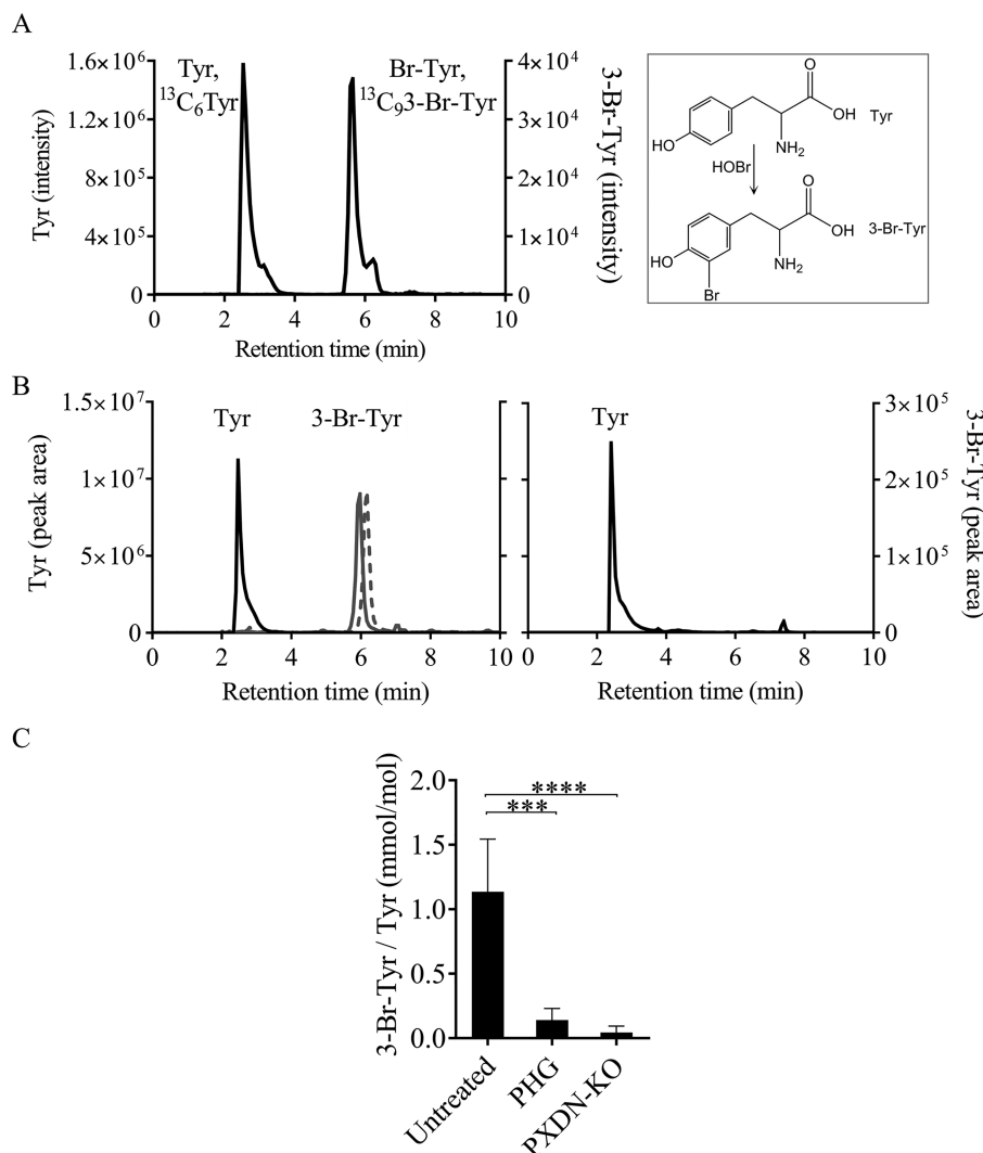
Figure 2. Identification of 3-Br-Tyr in extracellular matrix proteins using LC-MS/MS. A, typical LC-MS/MS chromatogram obtained in multiple reaction monitoring mode for the analysis of Tyr and 3-Br-Tyr. The retention time for ^{12}\text{C} -Tyr ( m/z 182 \rightarrow 136) and isotopically labeled ^{13}\text{C}_6 -Tyr ( m/z 188 \rightarrow 142) was 2.5 \pm 0.2 min. The retention time for the two isotopes ^{13}\text{C}_9 - ^{79}\text{Br} -Tyr ( m/z 260 \rightarrow 214) and ^{13}\text{C}_9 - ^{81}\text{Br} -Tyr ( m/z 262 \rightarrow 216) as well as the isotopically labeled internal standards ^{13}\text{C}_9 - ^{79}\text{Br} -Tyr ( m/z 269 \rightarrow 222) and ^{13}\text{C}_9 - ^{81}\text{Br} -Tyr ( m/z 271 \rightarrow 224) was 6.0 \pm 0.2 min. Artfactual bromination of ^{13}\text{C}_6 -Tyr was monitored by measuring ^{13}\text{C}_6 - ^{79}\text{Br} -Tyr ( m/z 266 \rightarrow 220) and ^{13}\text{C}_6 - ^{81}\text{Br} -Tyr ( m/z 268 \rightarrow 222). Chromatograms for isotopically labeled analytes were superimposable on their unlabeled counterparts. The chemical structure of tyrosine and 3-bromotyrosine are shown next to the chromatogram. B, representative chromatograms for tyrosine (solid black line) and two bromine isotopes of 3-bromotyrosine (solid gray line and dashed gray line, offset by 0.2 min for visibility) in ECM isolated from WT (left panel) or peroxidasin-knockout PFHR9 cells (right panel). The ECM samples were hydrolyzed with methane sulfonic acid then analyzed by LC-MS/MS. C, the levels of 3-Br-Tyr in ECM isolated from PFHR9 cells cultured for 6–8 days in the absence (Untreated) or presence of PHG, or isolated from peroxidasin-knockout PFHR9 cells (PFXDN-KO) calculated using standard calibration curves normalized to isotopically labeled internal standards. Values are the means of \geq 3 independent biological repeats \pm S.D. ****, p < 0.0001 ; ***, p < 0.001 by one-way ANOVA analysis followed by Tukey's multiple comparisons.
