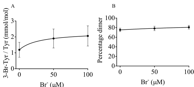
Figure 3. Effect of bromide supplementation on the formation of 3-Br-Tyr and sulfilimine cross-links in the ECM during cell culture. A, 3-Br-Tyr and B, NCD dimers in ECM isolated from PFHR9 cells cultured for 6–8 days with the indicated concentrations of bromide. Samples were analyzed as described in Figs. 1 and 2. Values are the means of \geq 3 independent biological repeats \pm S.D. Curves represent nonlinear regression lines selected to give best fit to the experimental data points.
