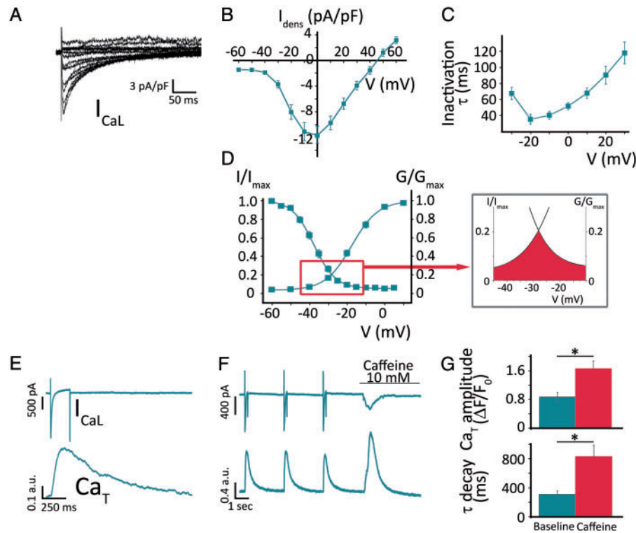
Figure 3 Ca^{2+} handling in Pluricyte ® CMs. (A) Voltage-dependent I_{CaL} activation; representative family of traces. (B) I_{CaL} -density I–V relationship ( n = 14 ). (C) Kinetics of inactivation of I_{CaL} (single exponential fit). (D) Steady-state activation and inactivation, fitted by Boltzmann equation. The inset depicts window I_{CaL} . (E) Simultaneous recordings of I_{CaL} and Ca^{2+} -transients ( Ca_T ) as a representative example. (F) Effect of caffeine (10 mmol/L) on membrane current and Ca_T , in a Pluricyte ® CM. (G) Average values of Ca_T amplitude (above) and decay time constant (below), at baseline and during caffeine perfusion.
