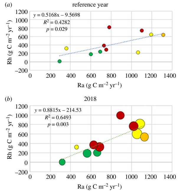
Figure 7. (a) Heterotrophic respiration (Rh) plotted against autotrophic respiration (Ra) for the respective reference year (see electronic supplementary material Table S2). (b) Similar plot but for the year 2018. The colour code as in figure 2. The size of the symbols for 2018 corresponds to the magnitude of the relative precipitation deficit (see also legend in figure 8). (Online version in colour.)
