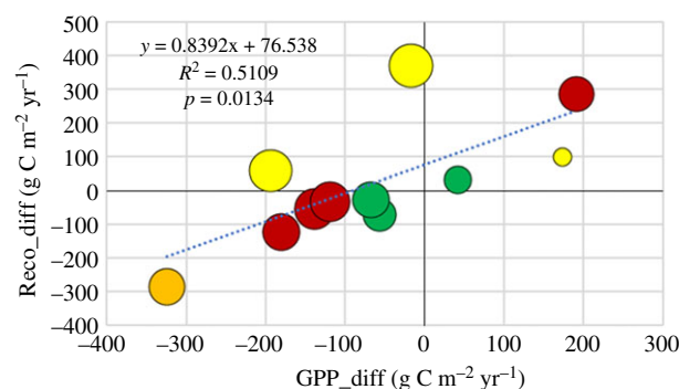
Figure 11. The anomaly in ecosystem respiration, Reco_diff, versus the anomaly in gross primary productivity, GPP_diff. Symbols as in figure 8. (Online version in colour.)
