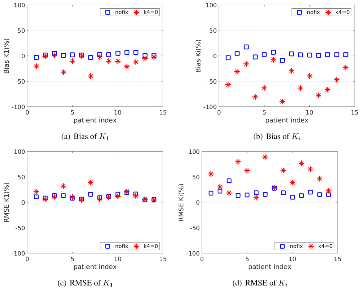
Figure 10. Bias and RMSE of K_1 and K_i of the fitting approaches with and without fixing k_4 at zero.
