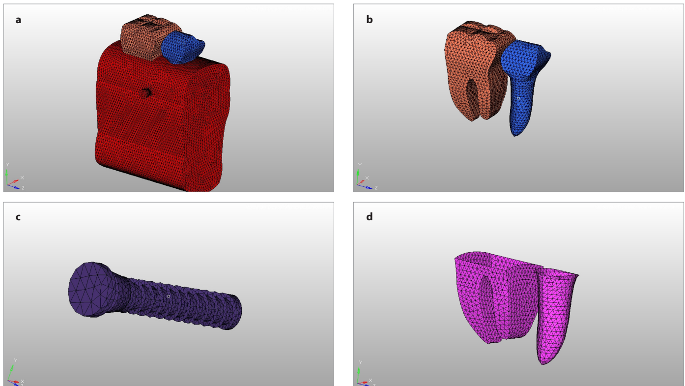
Figure 1. a-d. (a) FEM consisting of (b) tooth, (c) MI, (d) periodontal ligament and bone elements. FEM: finite element model
