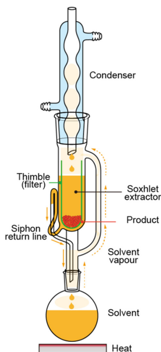
Fig. 20. Schematic illustration of Soxhlet extractor.
