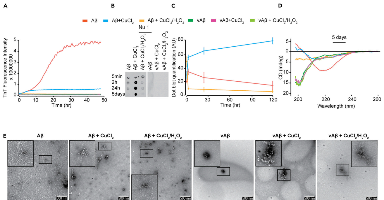
Figure 2. Metal-Catalyzed Oxidation Results in the Formation of Stabilized A \beta Assemblies
