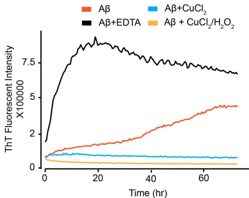
Figure S2. Related to Figure 1. Thioflavine T fluorescence assay comparing A \beta 1-42 self-assembly under MCO conditions, copper alone and in buffer with EDTA to chelate trace metals. A \beta 1-42 self-assembly at a higher rate than A \beta 1-42 in buffer suggesting that the trace metals present in the water used to make the buffer can influence the assembly rate.
