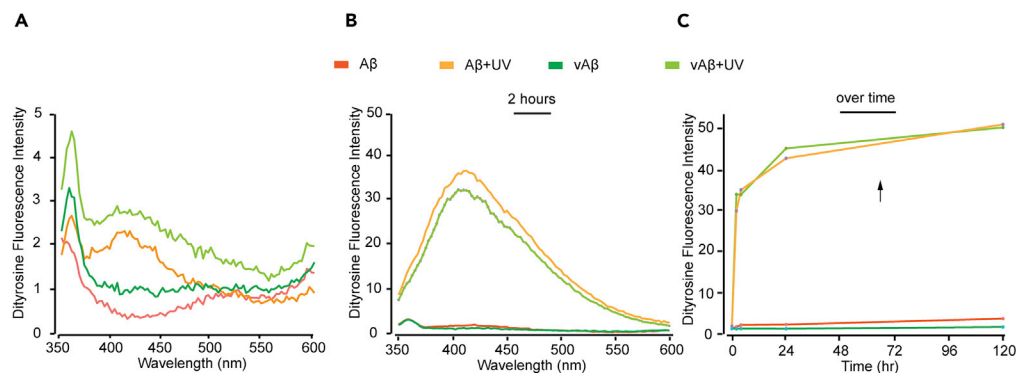
Figure 3. DiY Formation in A \beta and vA \beta via UV Photo-oxidation
