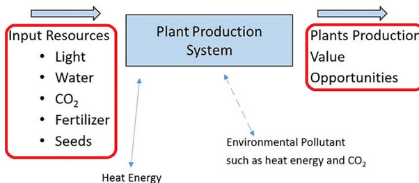
Fig. 1 Resource use efficiency (RUE) concept of a plant production system.
