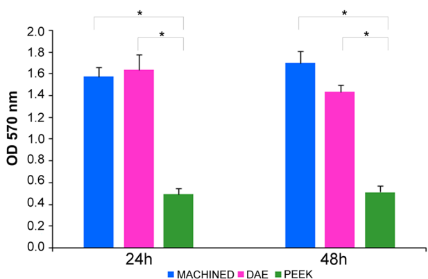
Fig. 6 Comparison of total biofilm biomass for the studied S. oralis biofilm developed on titanium discs machined, DAE and PEEK ones, after 24 and 48 h of incubation (error bars = ± standard deviation), determined by crystal violet staining (* p -value < 0.05)
