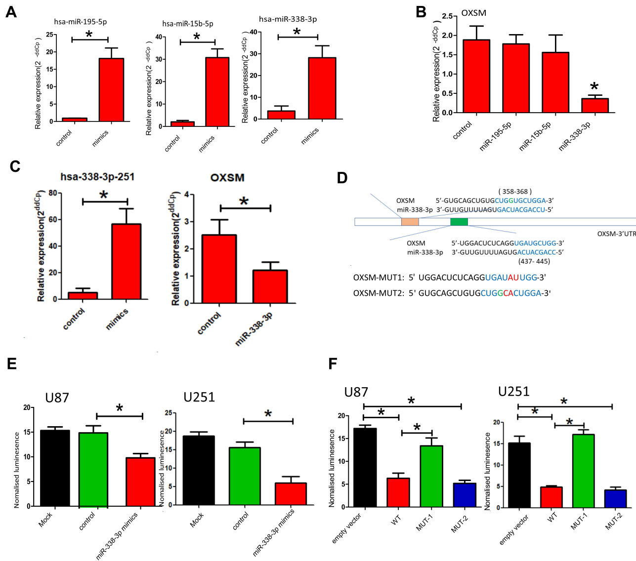
Figure 4 Identification of OXSM as direct target of hsa-miR338-3p . (A) hsa-miR195-5p , hsa-miR15b-5p and hsa-miR338-3p were overexpressed in the U87 cell lines by transfecting miRNA mimics; (B) the expression of OXSM in the U87 cell lines after transfecting of miRNA mimics; (C) hsa-miR338-3p were overexpressed in the U251 cell lines by transfecting miRNA mimics and the expression of OXSM in the U251 cell lines after transfecting of miRNA mimics; (D) the two putative binding sites between OXSM 3'UTR and hsa-miR338-3p ; Luciferase report vectors carrying the full OXSM 3'UTR of mutation site 1 (MUT-1, 437–445) and mutation site 2 (MUT-2, 358–368); (E) luminescence in hsa-miR338-3p -treated cells with wild-type reporters; (F) luminescence in hsa-miR338-3p -treated cells with MUT-1 and MUT-2 reporters. * P < 0.05 .
