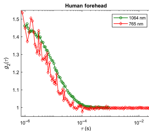
Fig. 8 g_2 measurements at 765 nm (red diamonds) and 1064 nm (green circles) on the forehead of a human subject. The 1064-nm measurements show a later decay and significantly higher SNR.
