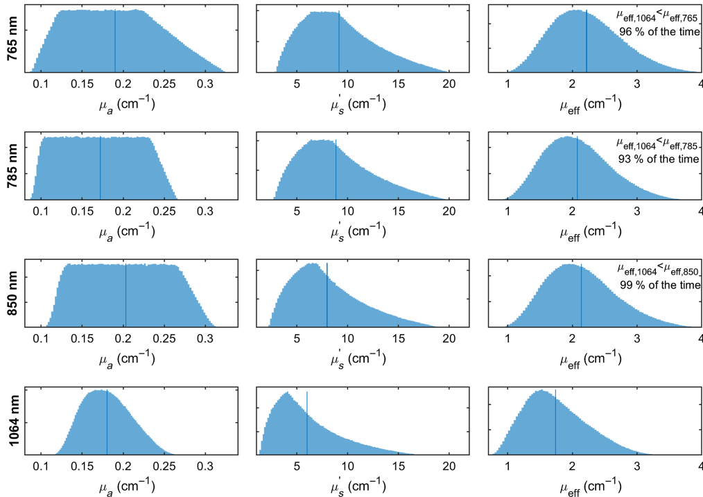
Fig. 2 Histograms of absorption, reduced scattering, and effective attenuation coefficients at 765, 785, 850, and 1064 nm, respectively, randomly sampled ( N = 150,000 ) for 40 \mu\text{M} < \text{HbT} < 120 \mu\text{M} , 40\% < \text{SO}_2 < 85\% , 0.55 < f_{\text{H}_2\text{O}} < 0.95 , 0 < f_{\text{fat}} < 0.4 , 8 < a < 25 , 0.5 < b < 2.4 to cover the vast majority of possible circumstances for tissue measurements. Vertical bars indicate average values. In pairwise comparisons (across the set of randomly sampled parameters), \mu_{\text{eff},1064} was lower than \mu_{\text{eff},765} , \mu_{\text{eff},785} , and \mu_{\text{eff},850} in 96%, 93%, and 99% of the time, respectively, indicating 1064 nm nearly always offers lower attenuation than the shorter wavelengths commonly used for DCS measurements.
