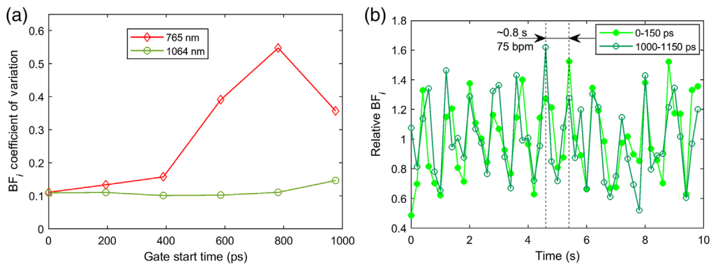
Fig. 10 TD-DCS comparison between 765 and 1064 nm. (a) Comparison of the BF_i CoV versus gate start time for TD-DCS measurements conducted at 765 nm (red diamonds) and 1064 nm (green circles) using a 1-cm source–detector separation and the maximum power allowed by regulatory standards. (b) Evidence of cardiac pulsation in BF_i at a 5-Hz acquisition rate for early (0 to 150 ps, light green filled circles) and late (1000 to 1150 ps, dark green open circles) gates.
