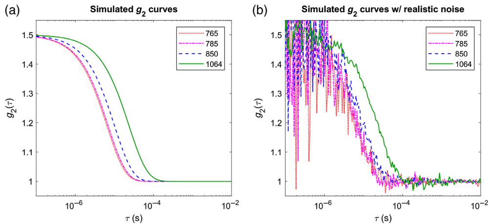
Fig. 3 Simulated g_2 curves for measurements with 3-cm source–detector separation on a homogeneous sample with optical properties matching Table 1, assuming \beta = 0.5 , an integration time of 10 s, and a blood flow index BF_i = 2 \times 10^{-8} \text{ cm}^2/\text{s} : (a) noise free; (b) with realistic noise added assuming a 7-kcps count rate at 765 nm, 8.05 kcps at 785 nm, 10.9 kcps at 850 nm, and 42.5 kcps at 1064 nm on each of 4 co-located fibers.
