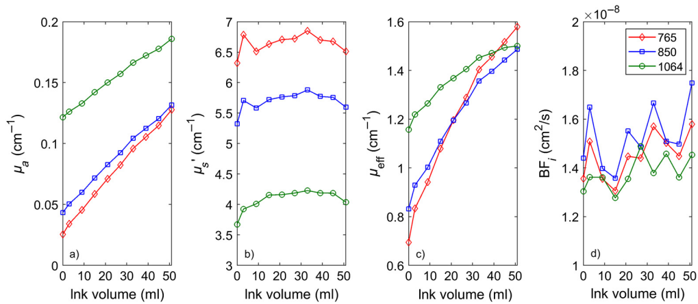
Fig. 6 CW-DCS measurements of BF_i (in this case, the Brownian diffusion coefficient D_b ) in a liquid phantom across wavelengths and phantom optical properties. (a) Optical absorption values, (b) corresponding optical scattering values, (c) corresponding attenuation coefficient values, and (d) recovered BF_i taking into account actual optical properties.
