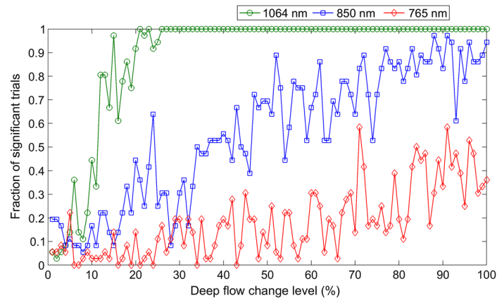
Fig. 4 Probability of detecting a statistically significant change in deep-tissue blood flow from a pair of 10 s measurements as a function of the actual amount of change for noise-realistic simulated measurements at 765 nm (red diamonds), 850 nm (blue squares), and 1064 nm (green circles). We assumed 30 \mu\text{M} HbT, with a 66% \text{SO}_2 , water fraction of 0.6 (no fat), and \text{BF}_i = 10^{-8} \text{ cm}^2/\text{s} for the superficial layer (1-cm thick), and 80 \mu\text{M} HbT with a 62.5% \text{SO}_2 , water fraction of 0.75 (also with no fat), and \text{BF}_i = 6 \times 10^{-8} \text{ cm}^2/\text{s} for the deep layer. The source-detector separation was set to 3 cm, and we assumed 7 kcps at 765 nm on four co-located fibers, scaling up to 10.9 and 42.5 kcps at 850 and 1064 nm, respectively, reflecting conservative estimates of the benefits of longer wavelengths.
