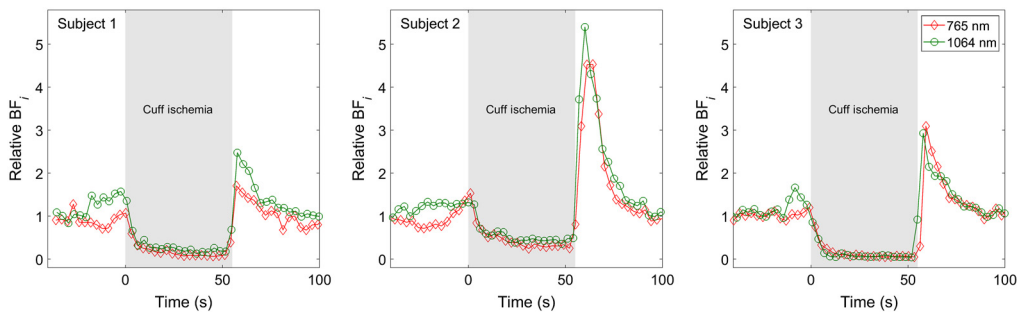
Fig. 7 Measurements of muscle blood flow before, during, and after an arm cuff occlusion maneuver in three different subjects. Measurements at 765 nm (red diamonds) and 1064 nm (green circles) were conducted one after the other. Despite the nonsimultaneous nature of the measurement, there is very good agreement between measurements taken in the same subject.
