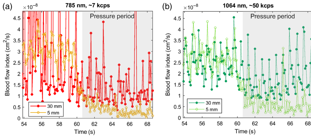
Fig. 9 CW-DCS BF_i time course measurements during pressure modulation maneuvers on the forehead of a human subject using a 10 Hz acquisition rate at (a) 785 nm (orange/red symbols) and (b) 1064 nm (light/dark green symbols), respectively. The short separation (5 mm: orange/light green open circles, respectively) BF_i decreases as expected during the pressure period and is no longer pulsatile; cardiac pulsation remains apparent in the long separation channel (30 mm: red/dark green filled circles, respectively) at both wavelengths; however, only 1064 nm offers sufficient SNR to resolve the pulsation at a 3-cm source–detector separation.
