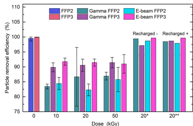
Fig. 1. Particle removal efficiency (PRE) as a function of the dose. Error bars represent the standard deviation. * - filters that were recharged with a negative surface potential, ** - filters that were recharged with a positive surface potential.
