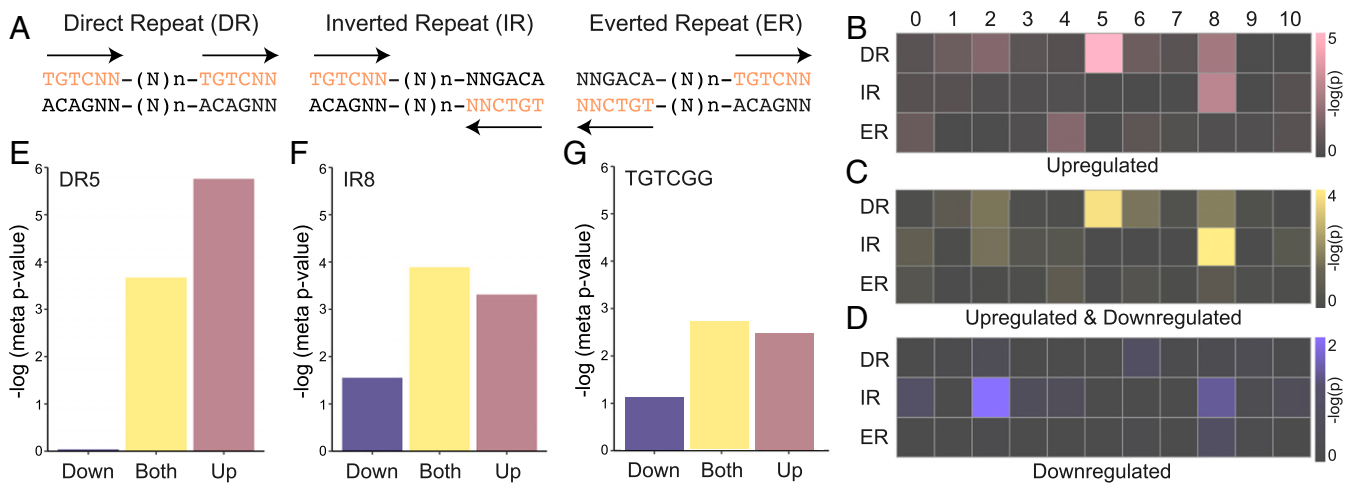
Fig. 3. Genome-wide association of AuxRE repeats with auxin responsiveness. (A) Definition of DR n , IR n , and ER n of TGTCNN hexanucleotide. N indicates A, C, G, or T. n indicates the number of nucleotides between two TGTCNN half-sites ( 0 \leq n \leq 10 ). (B–D) Association of DR n , IR n , or ER n variants present in the upstream regions (1,500 bp; 5'UTR) of the genes with auxin responsiveness. Color saturation visualizes the significance of overrepresentation for each composite element in -\log_{10}(\text{meta } p\text{-value}) units. Auxin-activated versus -nonactivated genes (B), both up- and down-regulated versus nonresponding genes (C), and down-regulated versus noninhibited genes (D). (E–G) Significance levels for association of DR5 (E), IR8 (F), and a single TGTCGG motif (G) with up-regulation, down-regulation, and both, in -\log_{10}(\text{meta } p\text{-value}) units.
