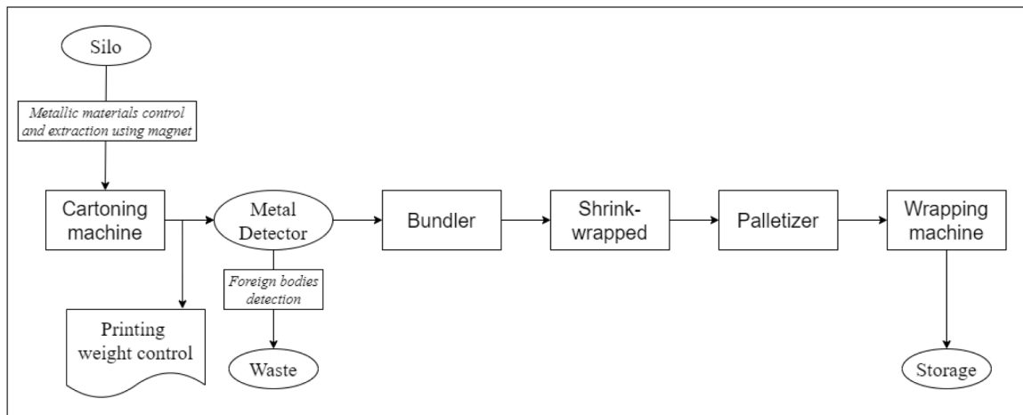
Fig. 3. Block diagram representing the “cardboard boxes line”.
