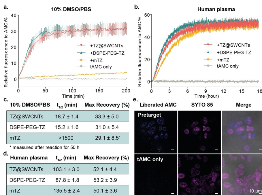
Figure 2. Tetrazine-responsive tAMC release. a,b) tAMC fluorescence recovery in response to TZ@SWCNTs, DSPE-PEG-TZ, or mTZ in 10% DMSO in PBS (a) and pure human plasma (b) measured by following the appearance of the fluorescence signal of AMC ( \lambda_{\text{ex}} = 380 nm, \lambda_{\text{em}} = 445 nm). The data represent the mean \pm STD ( n = 3 ). c,d) Calculated half-time of the tetrazine-responsive tAMC decaying reaction and maximum fluorescence recovery in 10% DMSO in PBS (c) and pure human plasma (d). e) Fluorescence imaging study of the pretargeted tAMC fluorescence activation in MCF-7 cells. The nuclei were stained with SYTO™ 85 orange; scale bar 10 \mu m.
