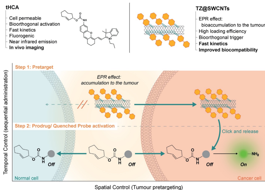
Figure 1. Illustration of the pretargeted strategy for selective activation in cancer cells. The approach takes advantage of the EPR effect-enabled accumulation of TZ@SWCNTs and the bioorthogonal IEDDA cleavage reaction between tetrazine and TCO to selectively deliver active therapeutic drugs or imaging probes to the tumour.
