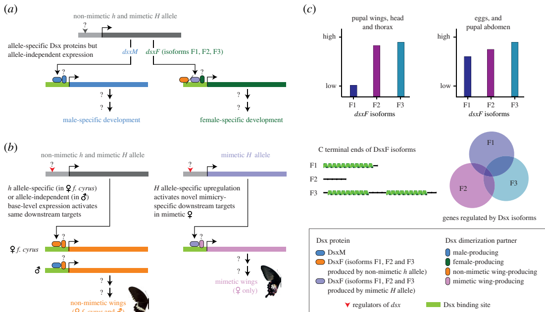
Figure 4. Proposed mechanism outlining the role of dsx in early-development sex differentiation and novel, late-development wing pattern polymorphism in Papilio polytes . (a) Early embryonic sex differentiation and late developmental sex-specific reproductive traits (e.g. genitalia and eggs) are highly canalized and strictly sex-specific, irrespective of allelic polymorphism and alternatively spliced isoforms [52,53]. (b) Late developmental novel mimetic wing patterns are produced by a combination allelic polymorphism, differential expression of alternatively spliced isoforms, and sex-limitation, expressing mimetic wing patterns only in females that contain at least one copy of the mimetic H allele of dsx (figure 2, [8,19,48]). (c) A graphic representation of relative Dsx isoform activity in regulation of polymorphic wings and other tissues (based on data from [8,19] and figure 3 from this study). Dsx F1 is downregulated in relation to F2 and F3 during the production of secondary sexual traits, but expressed comparably during sex differentiation and basic reproductive traits. The C terminal ends of the three DsxF isoforms are different (based on the electronic supplementary material, figure S2), and their downstream targets are probably different. The specific allelic variants [8,19], sex-specific and alternatively spliced Dsx proteins ([8,19] and the electronic supplementary material, figure S2 in this study), and molecular identities of downstream targets of dsx that regulate mimetic wing patterns ([48] and figure 2; electronic supplementary material, figure S1 in this study) have recently been identified. This model has several unexplored aspects that need to be studied in the future, including upstream regulators of dsx in each context, precise downstream targets, and both allele- and isoform-specific and protein-interacting partners of dsx . Such genes, regulators and networks with as yet unknown molecular genetic identities and mechanisms are marked with ‘?’.
