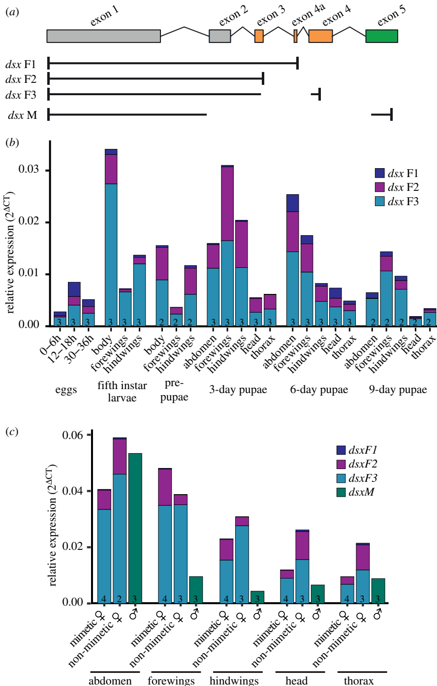
Figure 3. Expression of female isoforms of dsx in developing Papilio polytes . (a) dsx occurs as three isoforms in P. polytes females depending on the usage of female-specific exons 3 and 4. (b) Expression of female isoforms of dsx using qPCR. The number at the base of the bar indicates sample size for each tissue and stage. The female isoforms of dsx show different expression levels across tissues and stages, with F1 usually expressing at lower levels in most tissues compared to F2 and F3, which contribute to most of the dsx expression. (c) Expression of dsx isoforms in mimetic and non-mimetic female forms and males at 3-day pupal stage.
