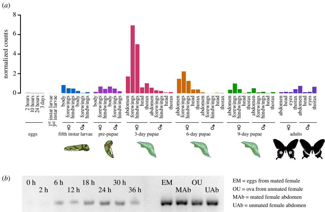
Figure 1. Expression of doublesex across developmental stages and tissues of Papilio polytes . (a) Expression of dsx from whole-transcriptome data of developing butterflies, from eggs to adults. Here, males represent non-mimetic wing patterns and females represent mimetic wing patterns. (b) dsx expression in eggs pre- and post-oviposition using RT-PCR. Of the four samples, MAb and UAAb corresponded to abdominal tissue of mated (MAAb) and unmated females (UAAb), excluding eggs and ova. The separated ovaries and eggs from abdominal tissue made up samples of eggs from mated (EM) and ova from unmated females (OU). 0 h eggs were freshly laid, and caterpillars usually hatched after 48 h.
