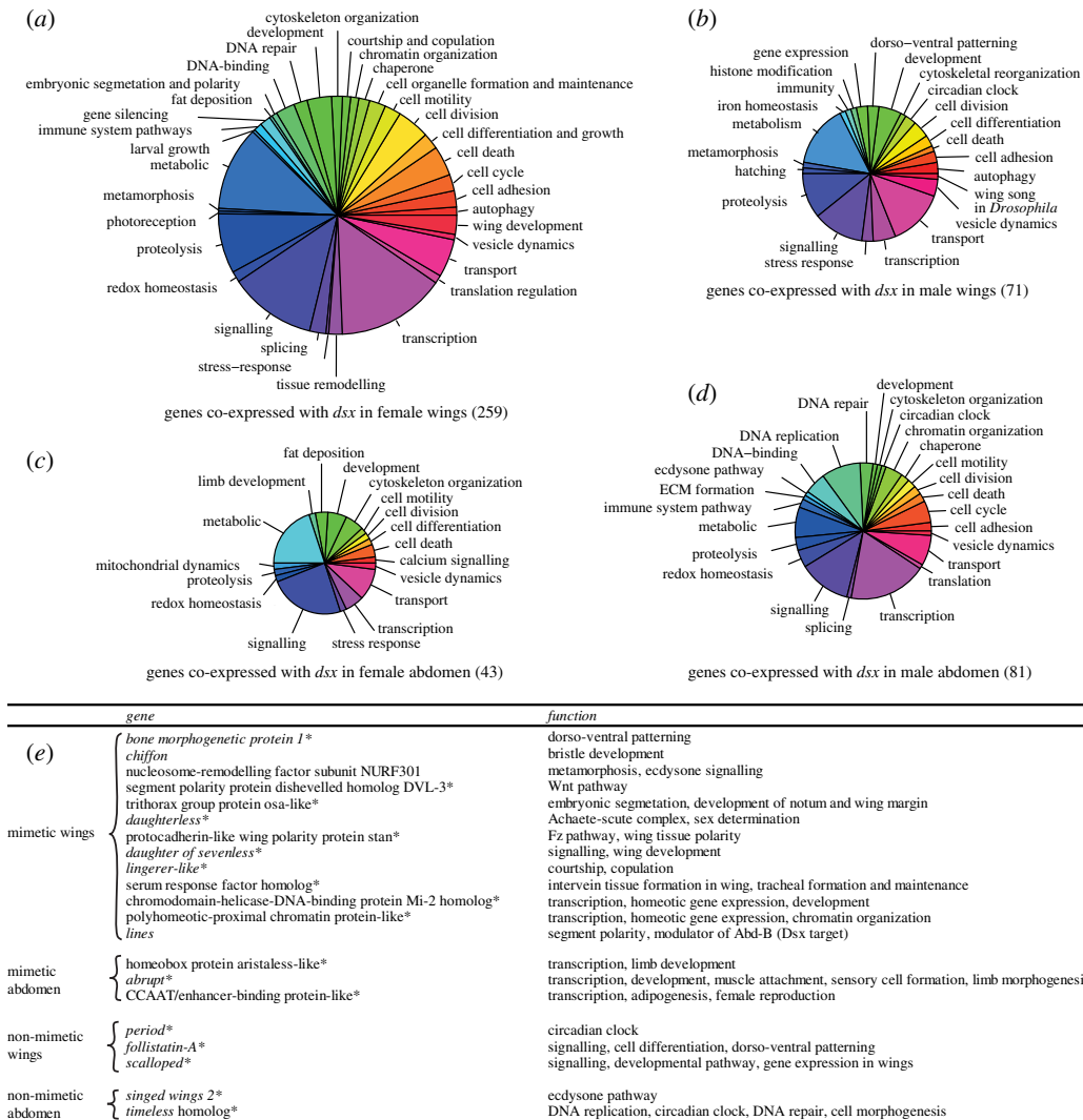
Figure 2. Putative targets of dsx in wings and abdominal tissue from co-expression analysis using WGCNA. Pie charts (a)–(d) depict functional categories of genes co-expressed with dsx in female wings, male wings, female abdomen and male abdomen respectively. Each pie chart is scaled by the number of genes that clustered with dsx in the same module. The table (e) highlights genes that are relevant in the context of wing development, patterning and reproduction in both mimetic and non-mimetic comparisons. Asterisk (*) denotes the presence of at least one dsx -binding motif in that locus.
