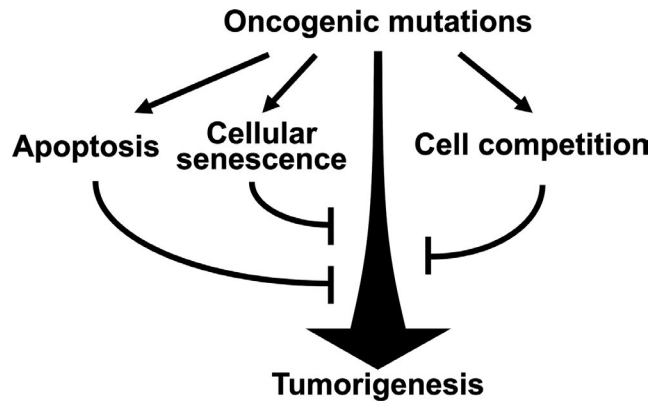
FIGURE 1 Oncogenic mutations trigger intrinsic tumor-suppressive programs. A variety of oncogenic mutations not only promote tumorigenesis but simultaneously activate intrinsic tumor-suppressive mechanisms such as induction of apoptosis, cellular senescence, and cell competition
