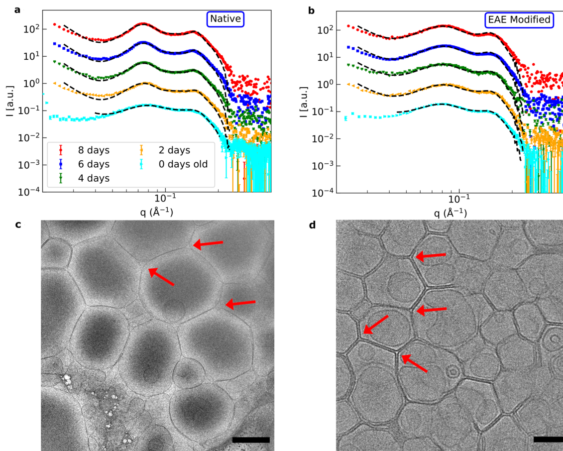
Figure 3. Kinetics of MBP-mediated assembly process followed by SAXS. SAXS data of (a) native and (b) EAE modified membranes mixed with 16.7 wt. ratio MBP 0, 2, 4, 6 and 8 days before the measurement. In (c) and (d) cryo-TEM pictures of aged native (5 days) and EAE modified (6 days) liposomes with 16.7 wt. ratio MBP are shown. The black bar in (c) corresponds to 500 nm and in (d) to 100 nm. For better visibility the different datasets in (a) and (b) have been vertically shifted. In (c) some of the rounded edges and in (d) some of the sharp edges have been marked by red arrows. The samples for SAXS and cryo-TEM were taken from the same batch for better comparison and had a lipid concentration of 5 mg/ml.
