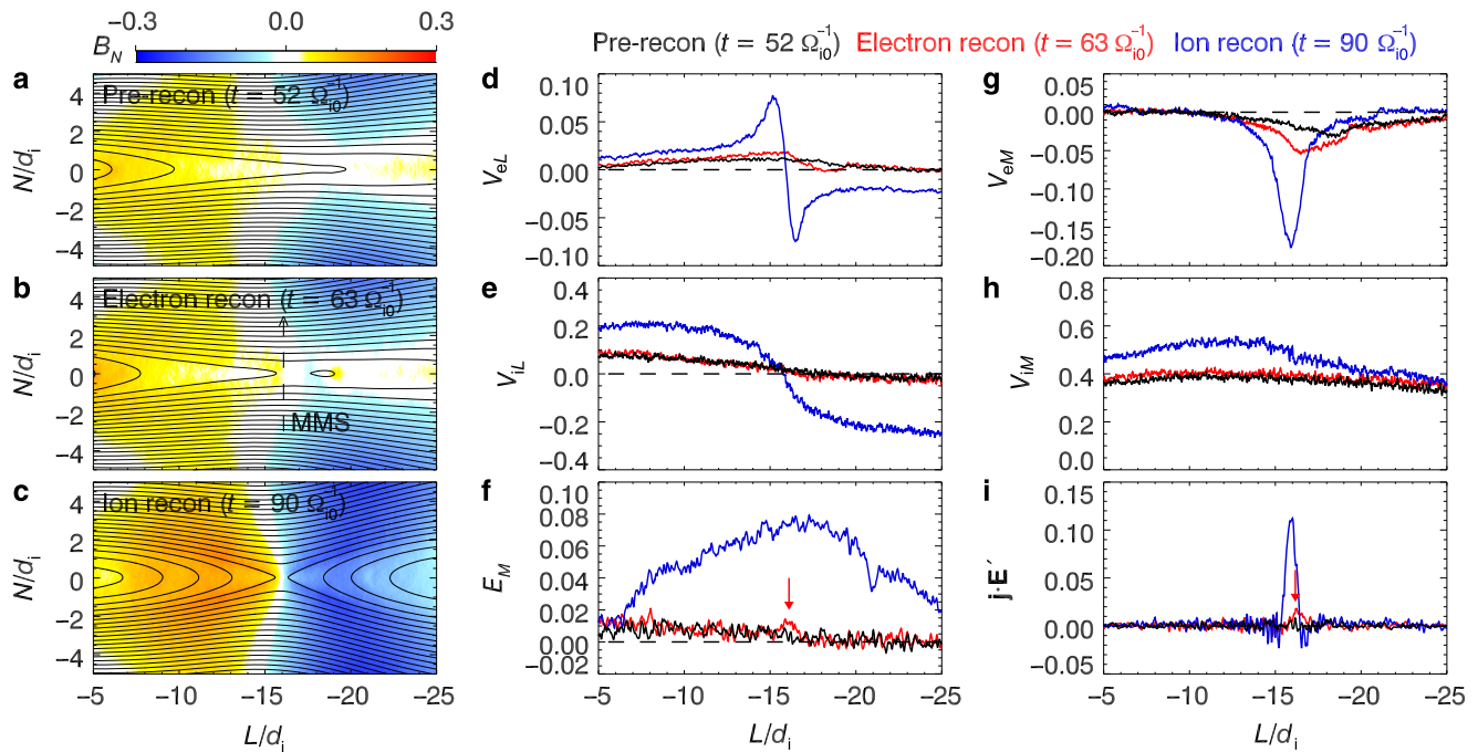
Fig. 3 PIC simulations of strongly externally driven onset of magnetotail reconnection. a–c Colors show the normal magnetic field B_N (in unit of B_0 ) in the L - N plane at pre-reconnection phase ( t = 52\Omega_0^{-1} ), electron reconnection phase ( t = 63\Omega_0^{-1} ), and ion reconnection phase ( t = 90\Omega_0^{-1} ), respectively. The black curves represent the magnetic field lines in the reconnection plane. d–i Profiles, along N = 0 , of V_{eL} (in unit of V_{eA} ), V_{iL} (in unit of V_{iA} ), E_M (in unit of V_A B_0 ), V_{eL} (in unit of V_{eA} ), V_{iL} (in unit of V_{iA} ), and \mathbf{j} \cdot \mathbf{E}' (in unit of e n_0 V_A^2 B_0 ) at pre-reconnection phase ( t = 52\Omega_0^{-1} , black curves), electron reconnection phase ( t = 63\Omega_0^{-1} , red curves), and ion reconnection phase ( t = 90\Omega_0^{-1} , blue curves). The dashed line with an arrow in b represents the virtual trajectory of the MMS spacecraft across the electron reconnection region, along L = -16.1d_i at t = 63\Omega_0^{-1} . The red arrows in f , i mark the location of the electron reconnection site.
