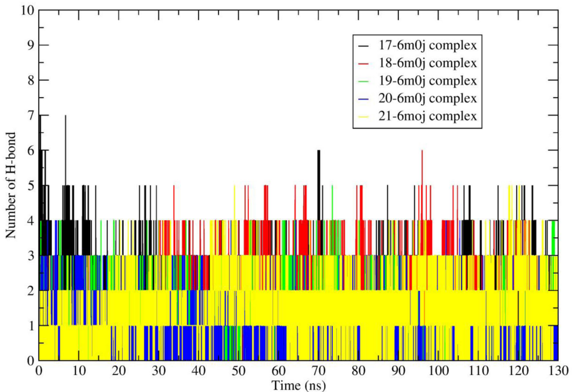
Figure 10. Number of average hydrogen bonding interactions between spike receptor–ligand (17–21) systems during 130 ns simulation time.
