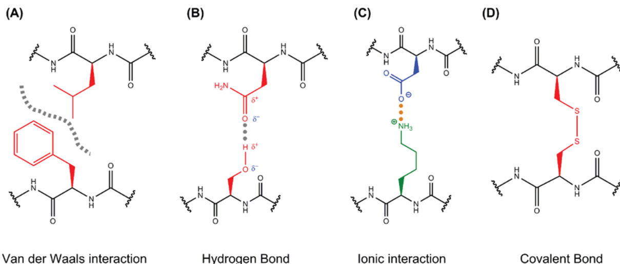
Figure 2. Intermolecular interactions
