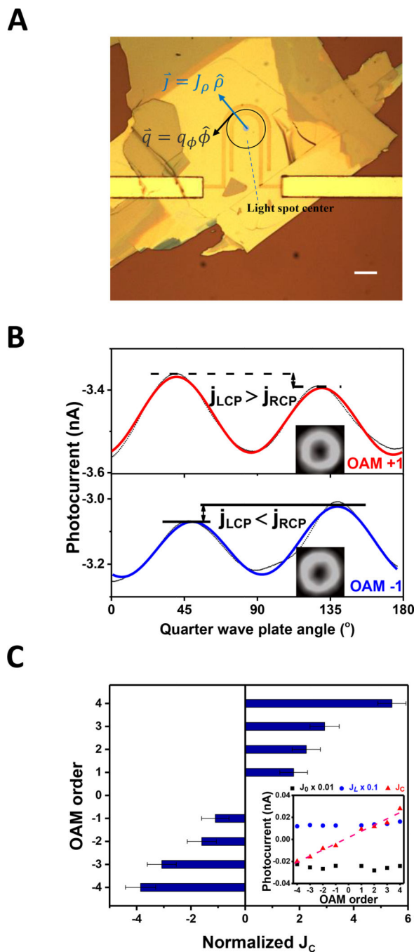
Figure 2: Evidence of the nonlocal photocurrent generated by OAM of light and its dependence on OAM order.
