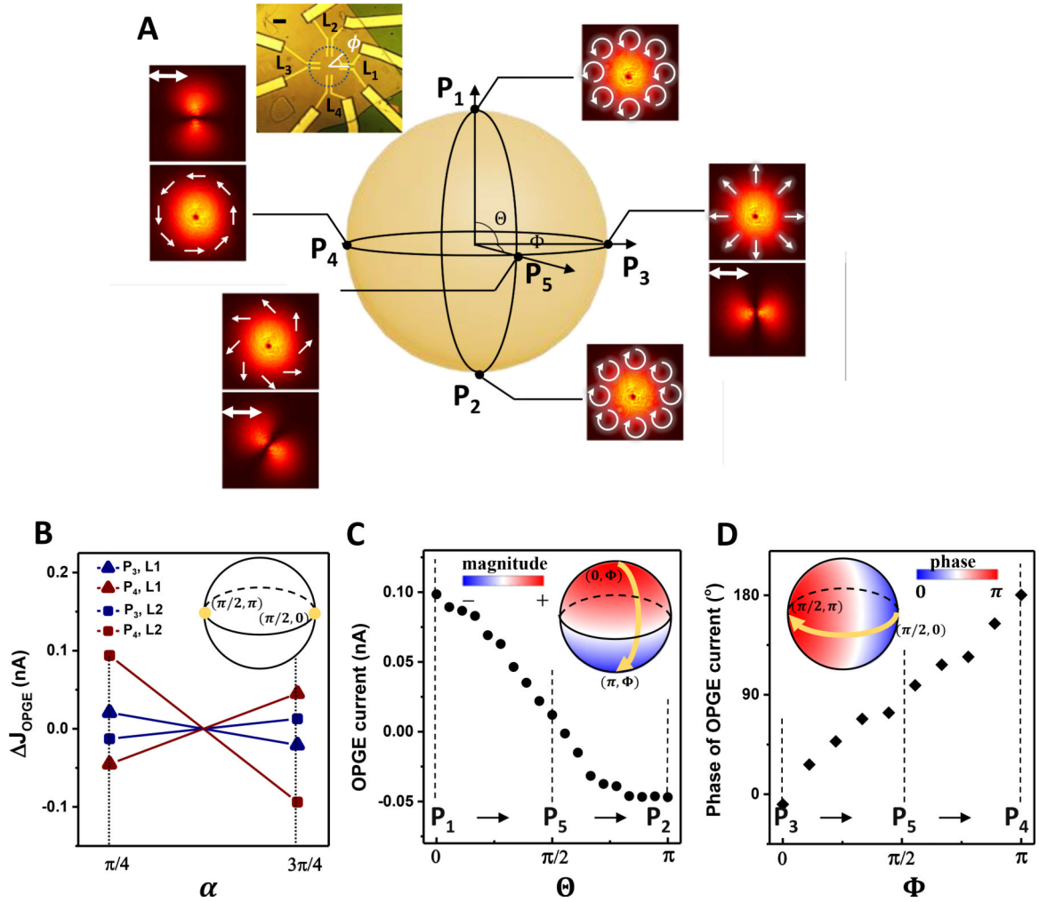
Figure 3: OPGE current from generalized vectorial OAM states on a HOPS.
