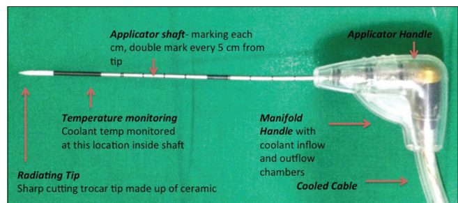
Figure 3: Microwave antenna
