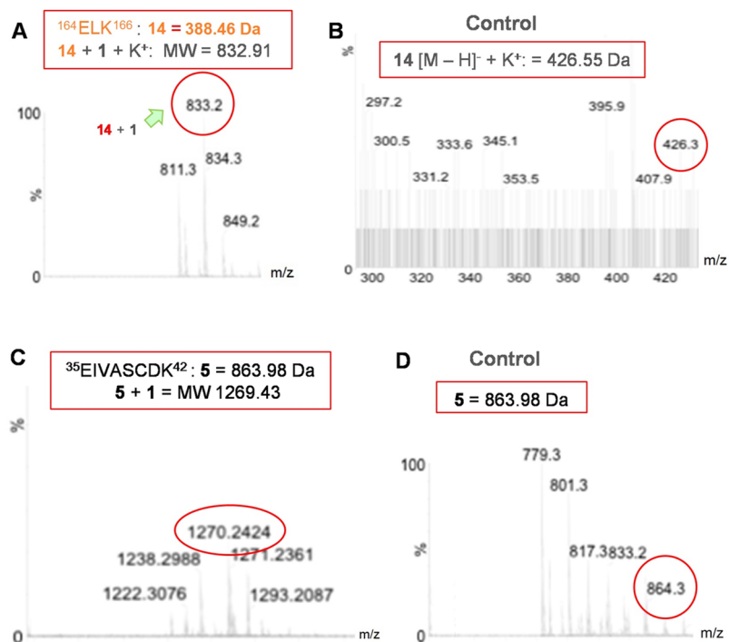
Figure 3. MS spectra of (A) fragment ^{164}\text{ELK}^{166} ( ^{157}\text{ELK}^{159} in regular HIV-1 IN) linked to photoprobe 1 , (B) its respective free peptide, (C) ^{157}\text{ELK}^{159} , ^{35}\text{EIVASCDK}^{42} + \mathbf{1} , and (D) the unlabeled peptide from the total tryptic digest of labeled HIV-1 IN + 1 conjugated.
