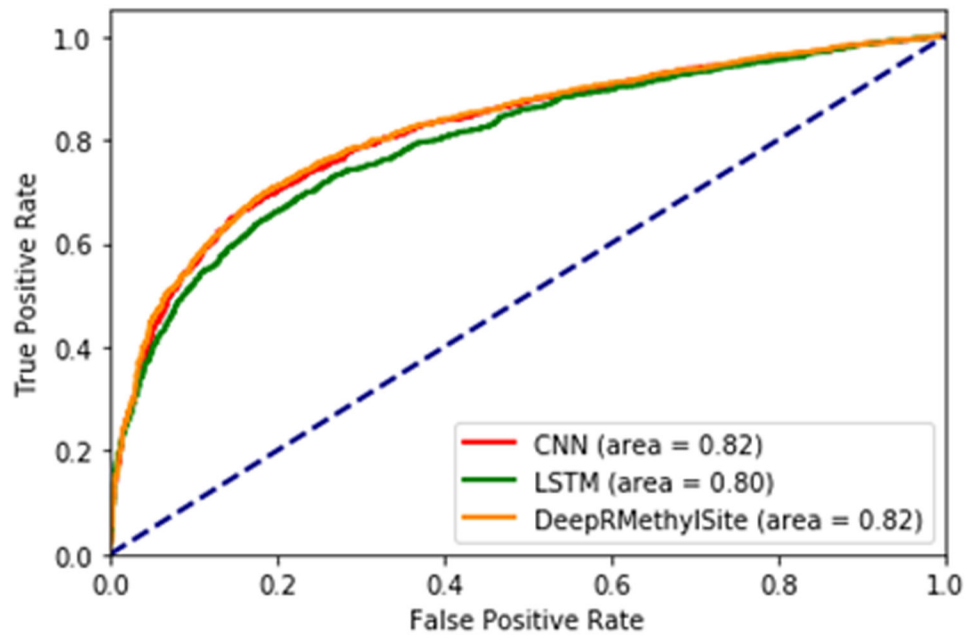
Figure 3: ROC Curve for LSTM, CNN and Ensemble model.
