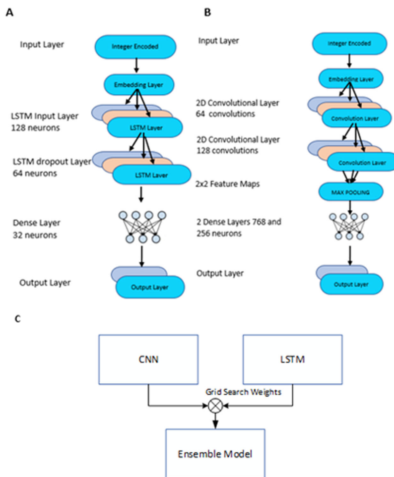
Figure 2: A. parameters used in LSTM model. B. Parameters used in CNN model. C. Ensemble model generated by combining through grid search weights on CNN and LSTM models.
