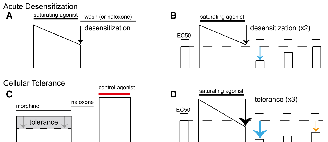
Fig. 1. Illustrations of electrophysiological experimental measures of desensitization and cellular tolerance. Desensitization is generally measured in two ways: first as in (A), an acute decrease in the response, usually a current or voltage measurement, in the continued presence of a saturating concentration of agonist over a period of minutes (generally 5–10 minutes). The extent of this decrease in signaling is acute desensitization (black arrow). Reversal of this signaling by agonist washout or application of antagonist is used to ensure that the baseline measurement has not changed during the experiment. The second measure of desensitization (B) is used in preparations such as cell culture or with agonists that can quickly be washed out of brain slices like [Met 3 ]enkephalin. First, a moderate concentration of agonist is applied to elicit approximately a half-maximal response (EC 50 ). Next, a saturating concentration of agonist is applied for minutes, similar to the protocol shown in (A), to desensitize the receptor (black arrow). The saturating agonist is washed out of the preparation, and then the EC 50 concentration of agonist is retested periodically to measure desensitization (cyan arrow) and the recovery from desensitization over time, which is nearly complete after 30–45 minutes. Cellular tolerance to chronic drug treatment is measured in several ways as well. (C) First, an agonist such as morphine is applied, and a response is measured; this is then reversed with an antagonist such as naloxone. Then, a control agonist that activates another receptor but ultimately activates the same downstream effector is tested (red bar). The relative response to morphine vs. the control agonist is measured. This is done in preparations from naïve animals (black line) or animals that have been chronically treated with morphine or other opioids for a period of days [generally 5–7 days (dotted line)]. The readout of cellular tolerance is a decrease in the response of morphine after chronic morphine treatment (gray shaded box, gray arrows) when normalized to the control agonist. (D) A second hallmark of opioid signaling in morphine-tolerant animals is an increase in desensitization after chronic morphine treatment. A protocol identical to that done in (B) is done on chronically morphine-treated mice; there is a characteristic increase in the decline in signaling in response to the saturating concentration of agonist (black arrow) as well as a smaller response to the EC 50 concentration after acute desensitization (cyan arrow). Furthermore, the rate of recovery from desensitization is prolonged, and the recovery from desensitization is incomplete (orange arrow).
