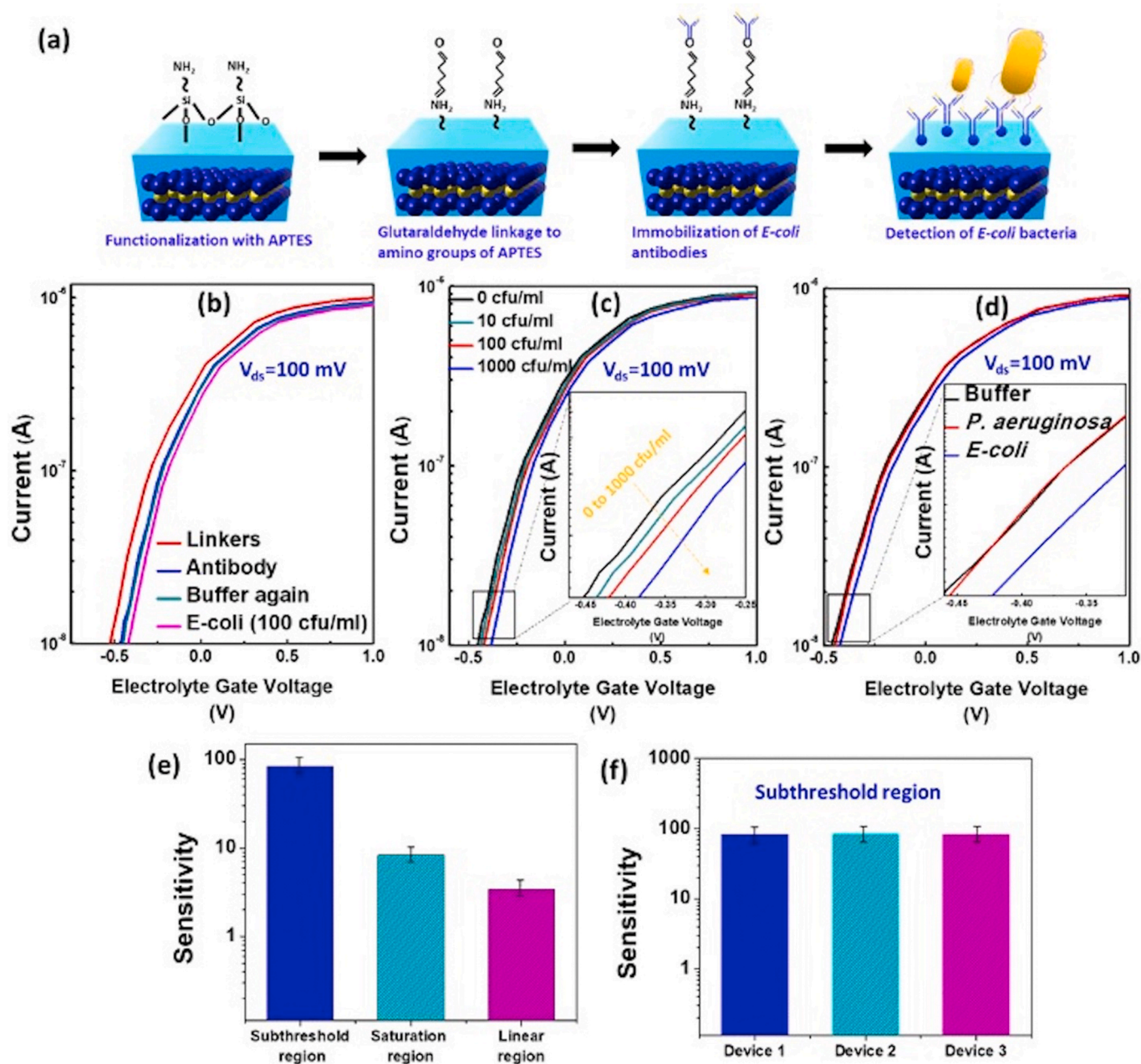
Fig. 4. E. coli bacteria detection on suspended MoS 2 FET: (a) Schematic diagram of self-assembly process for immobilization of E. coli bacteria on HfO 2 surface. (b) I_D - V_{LG} curve of SAM process at 100 mV bias; Functionalization of APTES (Red), immobilization of E. coli antibodies (Blue), buffer solution 0.01 M PBS solution of pH 7 (Cyan), and detection of E. coli bacteria of 100 CFU/mL (Magenta). (c) I_D - V_{LG} characterization of E. coli bacteria from 0 CFU/mL to 10 3 CFU/mL. (d) Comparison of I_D - V_{LG} characterization of E. coli and P. aeruginosa bacteria (100 CFU/mL) with PBS buffer solution. (e) Sensitivity measurement of E. coli bacteria at subthreshold, linear, and saturated regions. (f) Sensitivity comparison of three suspended MoS 2 FET devices by immobilizing the 100 CFU/mL E. coli bacteria. (For interpretation of the references to colour in this figure legend, the reader is referred to the Web version of this article.)
