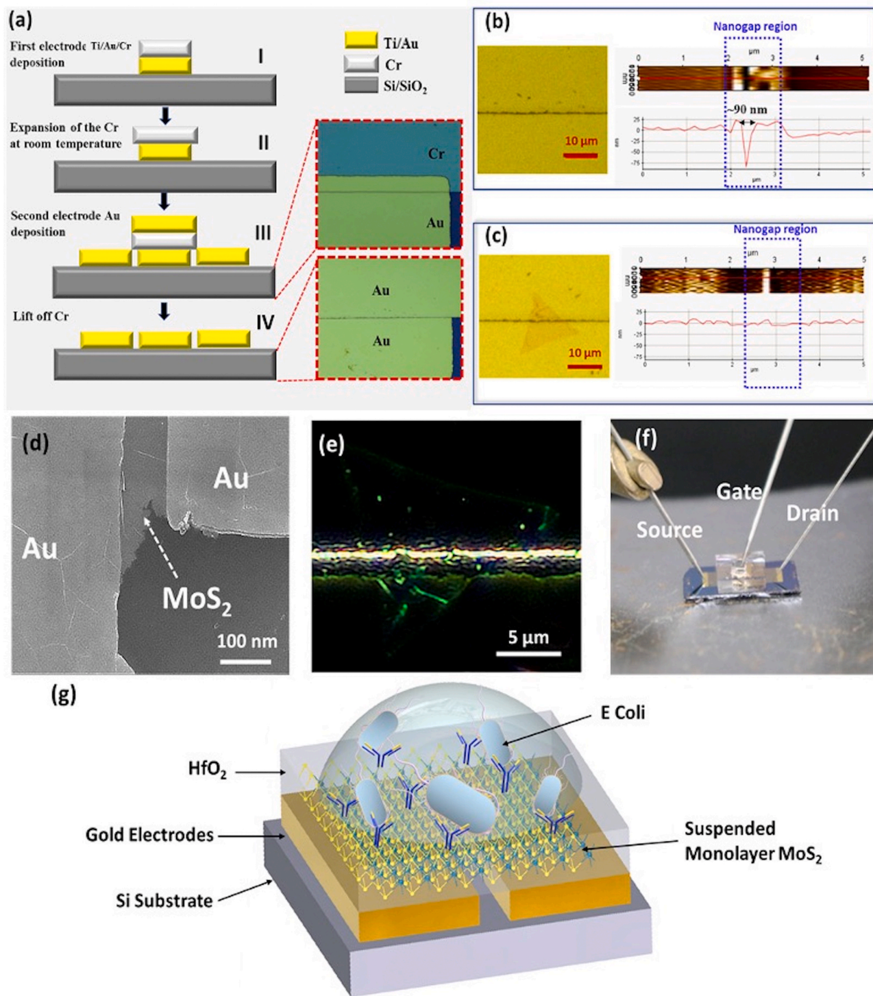
Fig. 1. Fabrication of suspended MoS 2 FET: (a) Schematic representation of the process flow to achieve nanogap electrodes. Optical image, AFM mapping, and line diagram of nanogaps (b) without MoS 2 (c) with MoS 2 . (d) high magnification SEM image of MoS 2 on the top of nanogaps (e) Optical dark field image of MoS 2 triangle on the top nanogaps. (f) Image of biosensor device with Source, Drain, and Gate (Ag/AgCl electrode) connection (g) Schematic of Biosensor with E. coli and antibodies.
