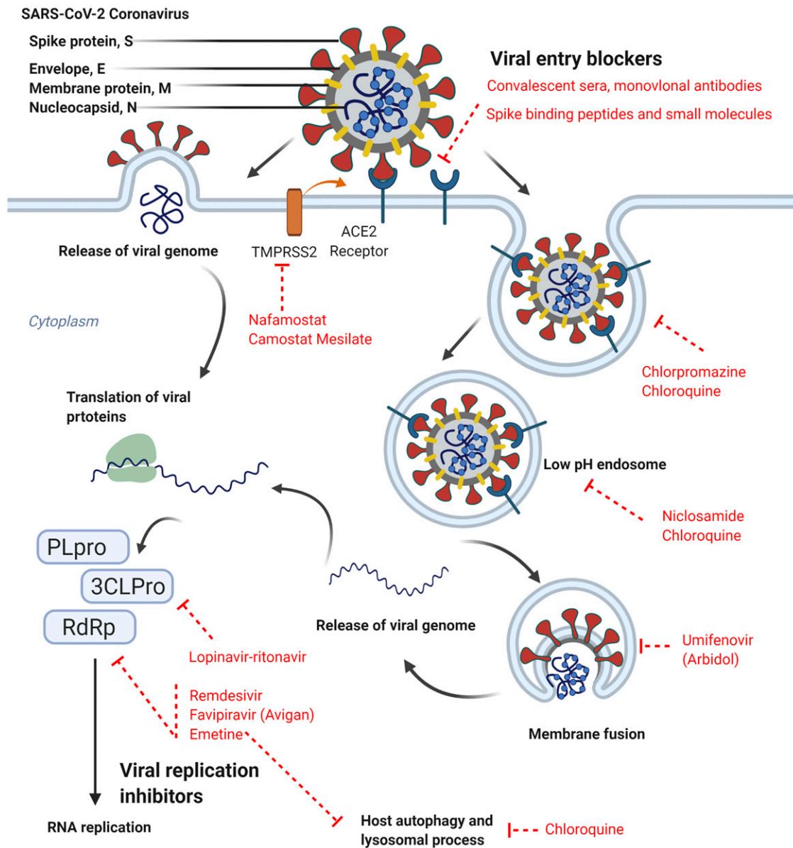
Fig. 1. SARS-CoV-2 spike (S) protein binds the cell surface receptor ACE2 on host cells. Viral genome is delivered into the host cytosol by 1) directly fusing with the plasma membrane after being cleaved and activated by the serine protease TMPRSS2 or 2) using the host cell's endocytic machinery in which the endocytosed virions are subjected to an activation step in the endosome. The viral genome also functions as the messenger RNA, which is translated into proteins, such as 3CLPro, papain-like cysteine protease (PLpro), and RdRp, by host cell machineries. The SARS-CoV-2 genome also encodes the structural proteins (S), envelope (E), membrane (M), and nucleocapsid (N). RdRp is essential for viral replication and therefore is an attractive target for anti-SARS-CoV-2 drugs. Drugs that are currently in clinical trials are shown here in red, along with their targets of viral life cycle or viral-host interactions. Figure created in BioRender.
