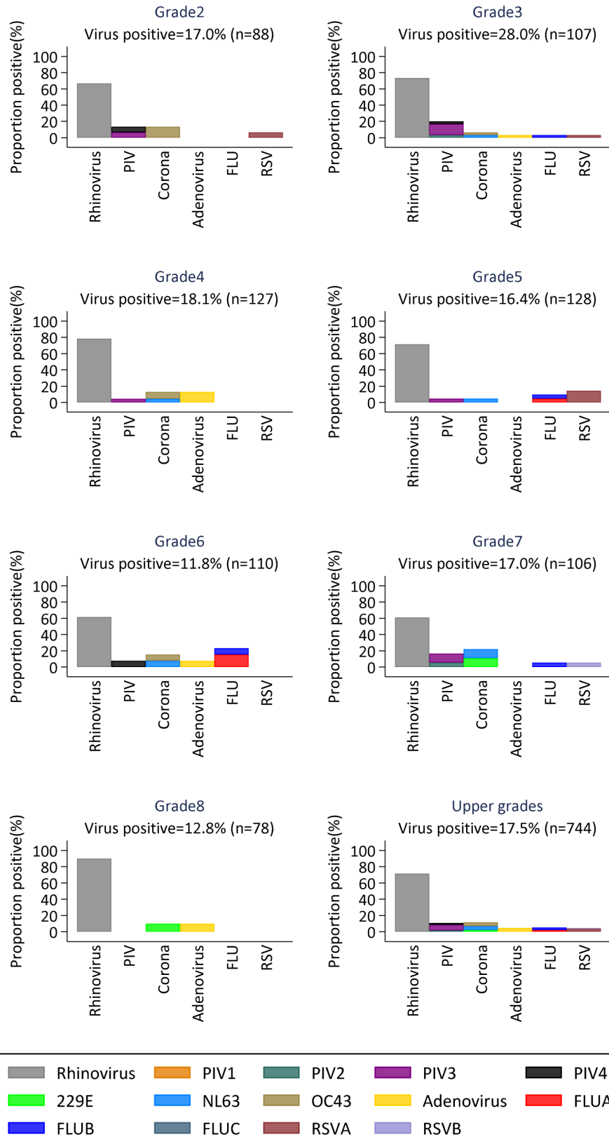
Figure 4. Proportions of virus positive samples in each of the grades in upper primary. Each panel shows the distribution of the six different virus groups per grade. (RSV- respiratory Syncytial Virus; FLU- Influenza virus A, B, C; PIV -Parainfluenza virus 1–4; Corona- Human coronavirus NL63, E229, OC43; Rhinovirus-Human rhinovirus).
