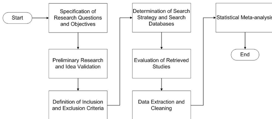
Fig. 1. Methodological flow diagram for the systematic review and meta-analysis.
