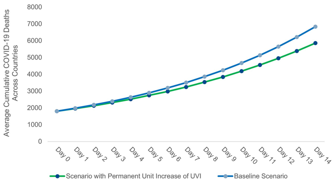
Figure 3. Long-run effects of a permanent unit increase of Ultraviolet index (UVI) on average cumulative COVID-19 deaths across countries.
