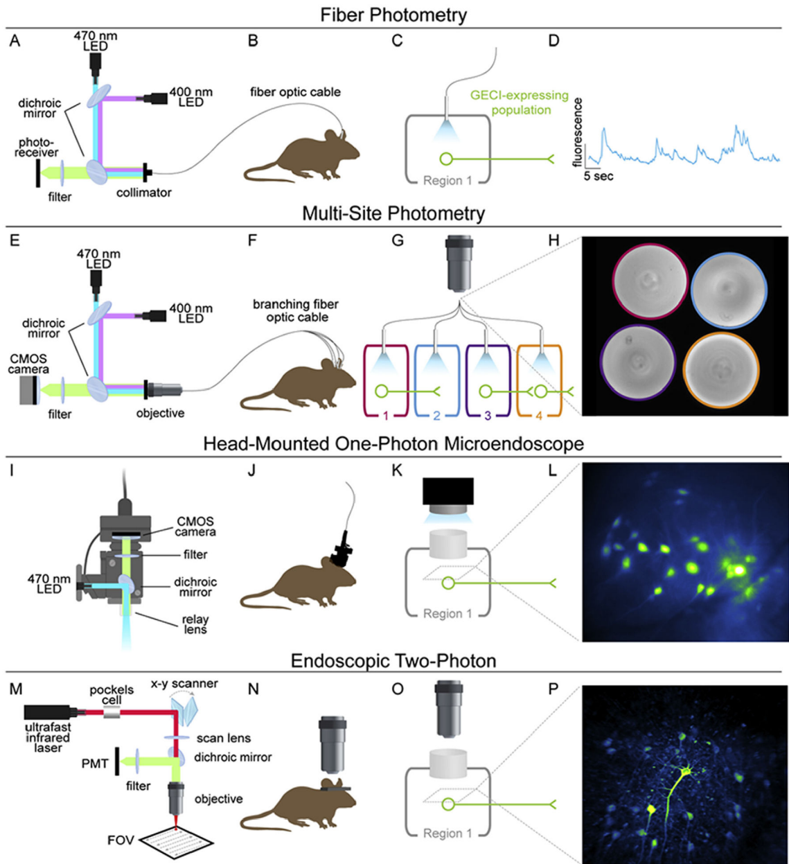
Fig. 1. Commonly used approaches for in vivo calcium imaging.
