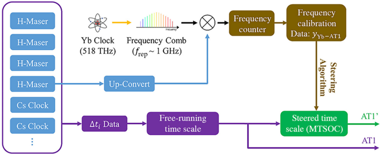
FIG. 2. Experimental scheme of optical-clock-based time scale \text{AT1}' and comparison to free-running time scale \text{AT1} .
