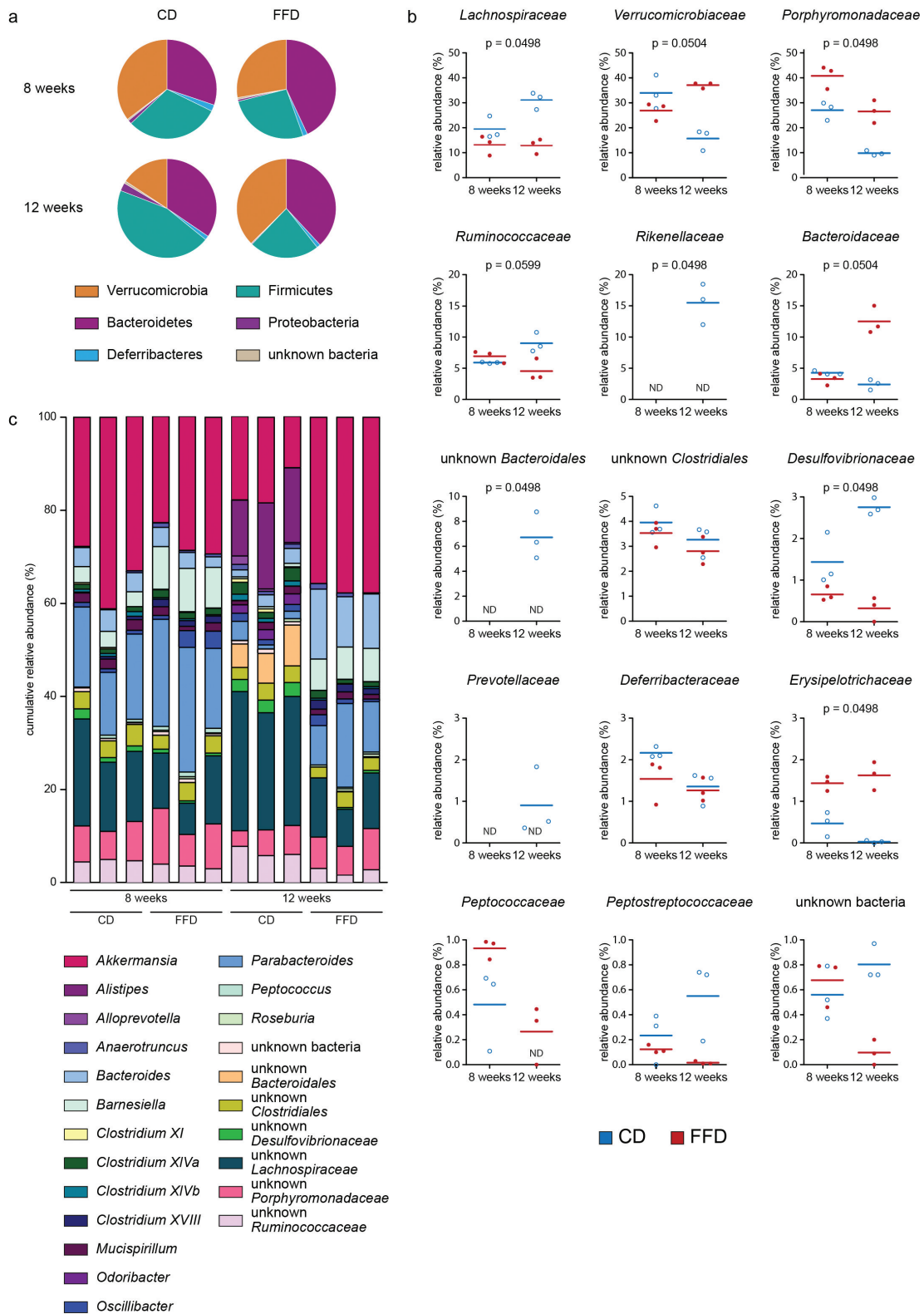
Figure 2. Alterations of intestinal microbiota at taxonomic levels. Taxonomic composition of the intestinal microbiota of CD or FFD mice. (a) Phyla, (b) family and (c) genera at the age of eight and twelve weeks was measured via 16S rRNA gene amplicon analysis ( n = 3 ). Statistical analysis: (b) Kruskal-Wallis Rank Sum Test for all groups (corrected for multiple comparison by Benjamini-Hochberg method). Data are shown as individual mice and means and are representative of two independent experiments.
