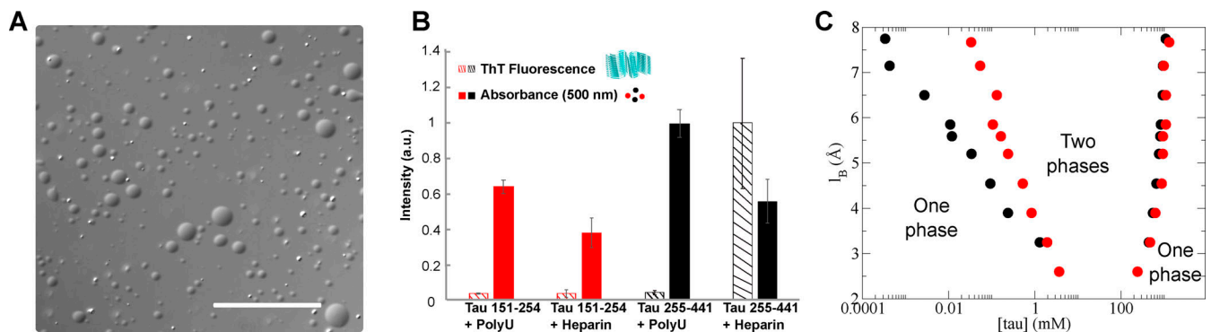
Figure 6. Similar to Tau 255–441, Tau 151–254 can form droplets in vitro . (A) Representative bright-field images of Tau 151–254/polyU droplets. Scale bar is 50 \mu\text{m} . (B) Direct comparison of Tau 151–254 (red) and Tau 255–441 (black) shows phase separation occurs for both protein segments with addition of PolyU or heparin. In contrast to the Tau 255–441 heparin complex, Tau 151–254 does not show the capacity to form fibrils with either PolyU or heparin. Turbidity was evaluated at 500 nm (filled bar); fibrilization was evaluated by ThT fluorescence (striped bar). Protein concentration was 50 \mu\text{M} , PolyU concentration (where applicable) was 125 \mu\text{g/ml} , and heparin concentration was 12.5 \mu\text{M} . All data were normalized by the largest measured value or absorbance or fluorescence. n = 3 ; error bar in SD. (C) Predicted Tau 151–254/RNA binodal phase coexistence points modeled using FTS. Calculations performed for Tau 151–254 (red dots) are compared with our previously reported (Lin et al., 2019) phase diagram for Tau 255–441 (black dots), showing that both sequences have a stable two-phase region under similar electrostatic environments and solvent conditions. The conditions for stable binodal phase coexistence depend on the strength of the electrostatic interaction, characterized in our model by the l_b as the input parameter. The region defined by the coexistence points is the region at which the system forms a thermodynamically stable droplet phase in coexistence with a solution phase. Areas corresponding to one-phase or two-phase are shown in the diagram.
