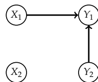
Figure 8. Graph of the model \mathcal{N}_{CIS} .
