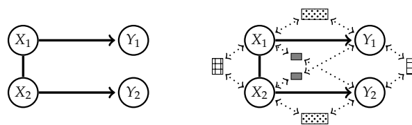
Figure A1. Starting graph and possible two way interactions.
