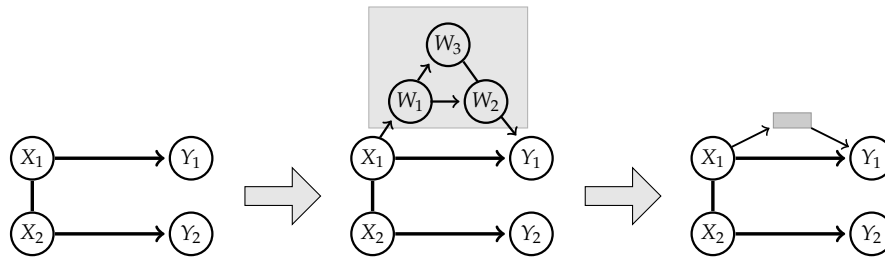
Figure 11. Example of an exterior influence on the initial graph.
