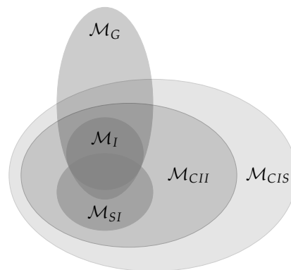
Figure 12. Sketch of the relationship between the manifolds corresponding to the different measures.
