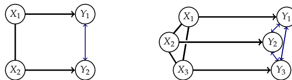
Figure 5. Marginalized Model for n = 2 and n = 4 .
