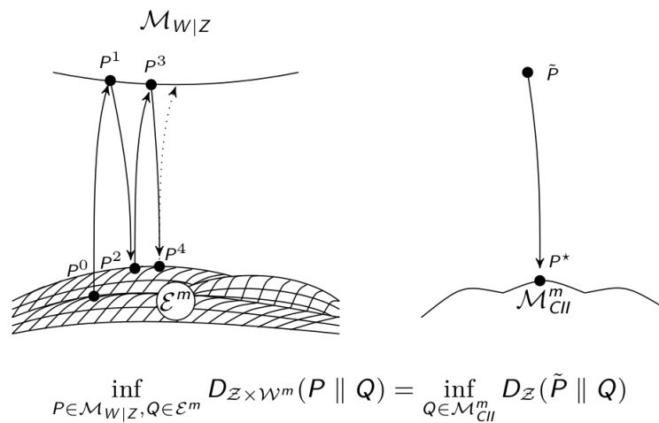
Figure 13. Sketch of the em-Algorithm.
