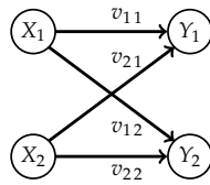
Figure 14. The weights corresponding to the connections for n = 2 .
