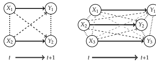
Figure 1. The fully connected system for n = 2 and n = 3 .
