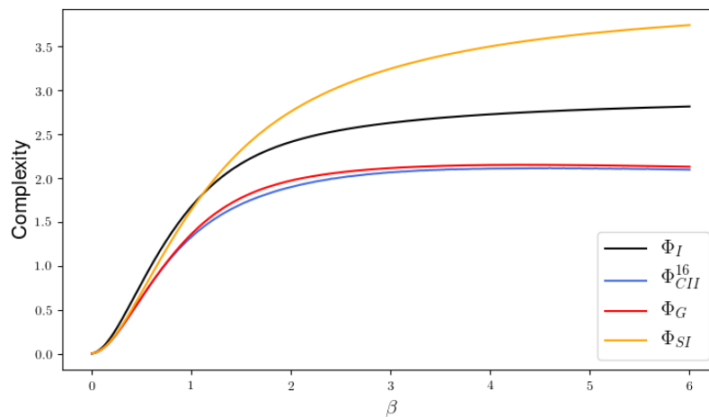
Figure 17. Ising model with 5 nodes.
