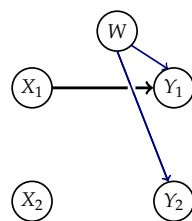
Figure 9. Graph of the model \mathcal{N}_{CII} .
