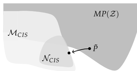
Figure 10. Sketch of the relationships among MP(\mathcal{Z}) , \mathcal{M}_{CIS} and \mathcal{N}_{CIS} .
