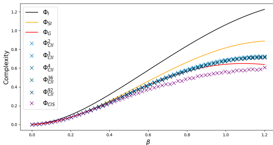
Figure 16. Ising model with 3 nodes.
