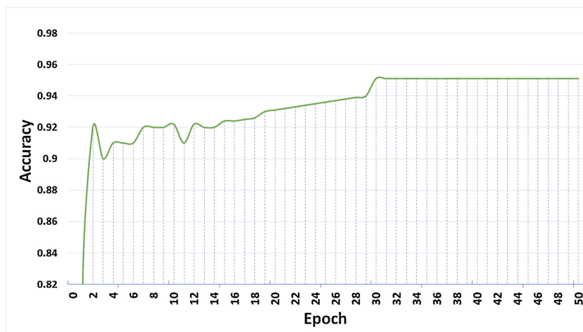
Fig. 11. Training Accuracy of YOLOv3 using overhead view data set.
