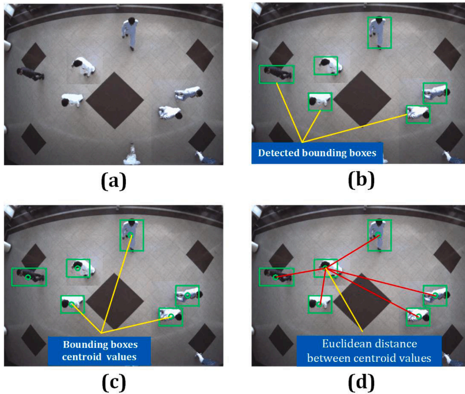
Fig. 8. (a) Input image, (b) detected person bounding boxes using deep learning algorithm, (c) compute the centroid of each detected bounding box, and (d) finally, the distance between each pair of the centroid is determined. In the example image, the red lines indicate the distance between each bounding box centroid. (For interpretation of the references to color in this figure legend, the reader is referred to the web version of this article.)
