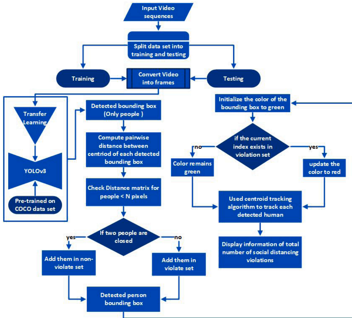
Fig. 5. Flow diagram of overhead view social distance monitoring framework.
