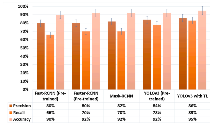
Fig. 15. Comparison results of YOLOv3 trained on overhead data set with other methods.
