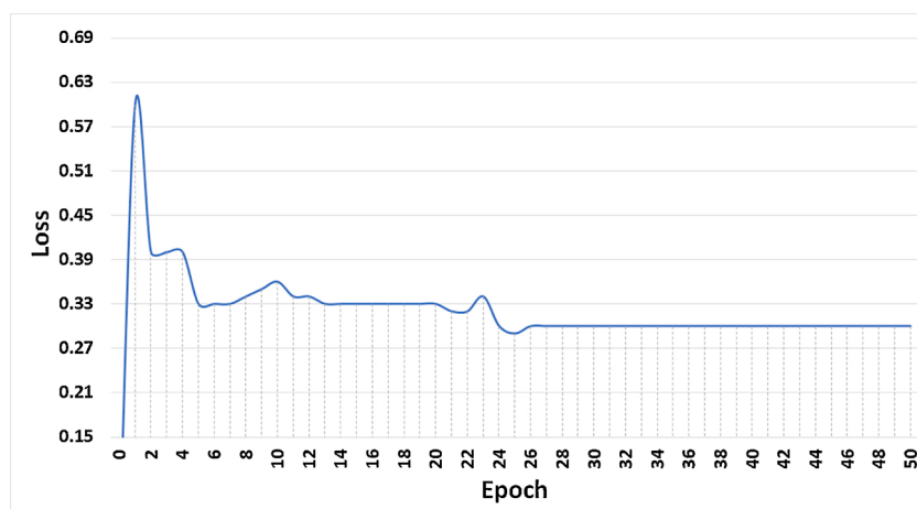
Fig. 10. Training loss of YOLOv3 using overhead view data set.
