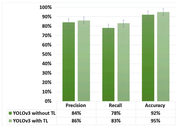
Fig. 13. Precision, Recall, and Accuracy of model (YOLOv3) with and without transfer learning.
