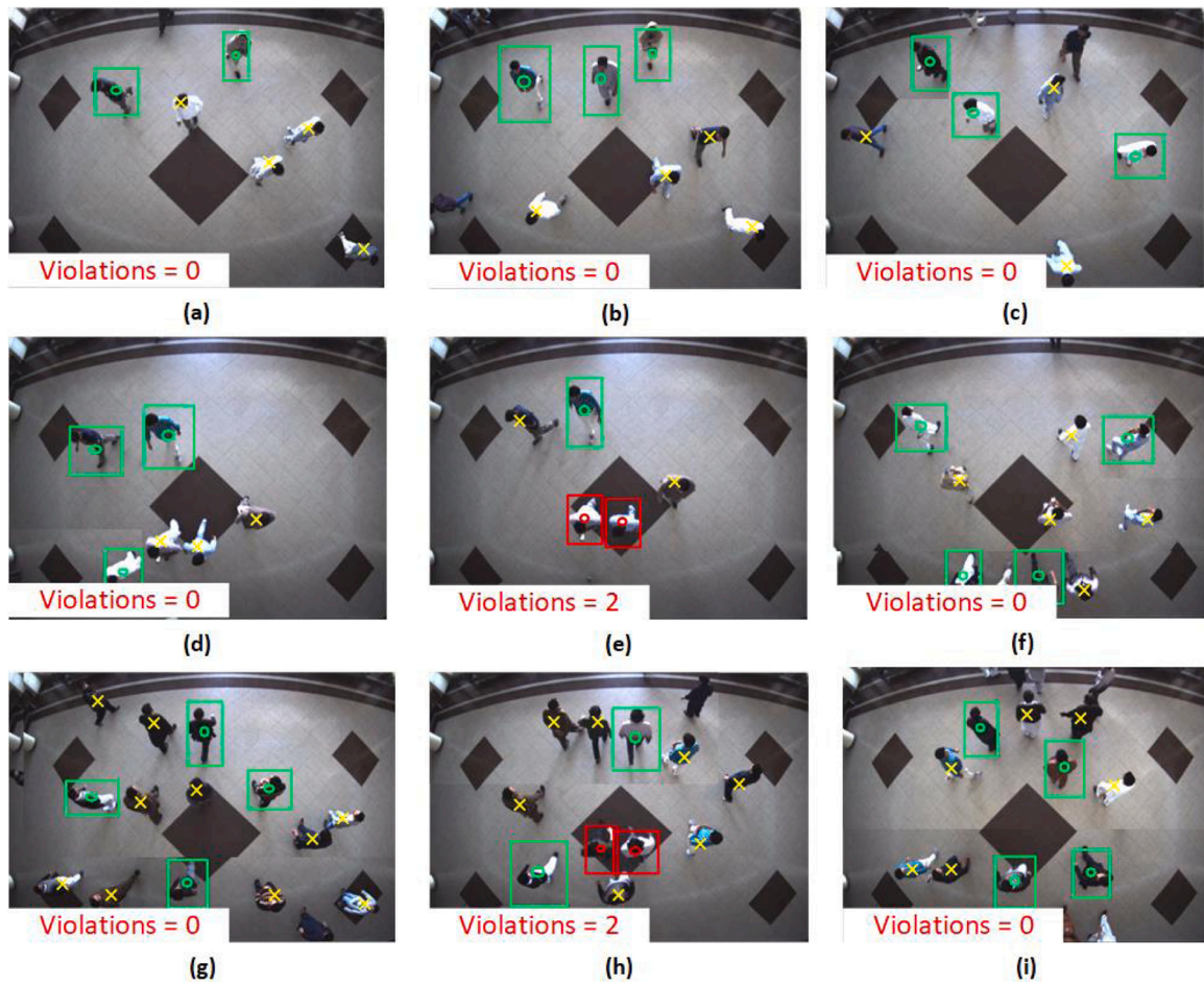
Fig. 9. Social distance monitoring from an overhead view using a pre-trained detection model. In sample frames, the people in green rectangles are those who maintain the social distancing. The people who violate the social distance threshold are shown red in rectangles. The manually labels yellow positive cross shows miss detections. (For interpretation of the references to color in this figure legend, the reader is referred to the web version of this article.)
