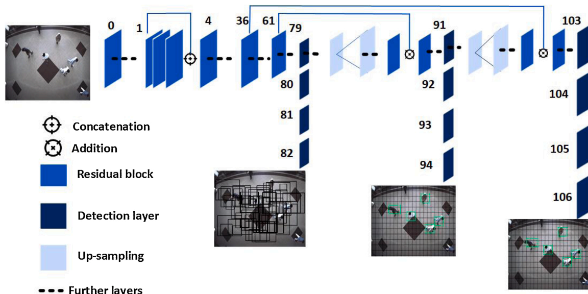
Fig. 6. General architecture of YOLOv3 utilized for overhead view human detection.
