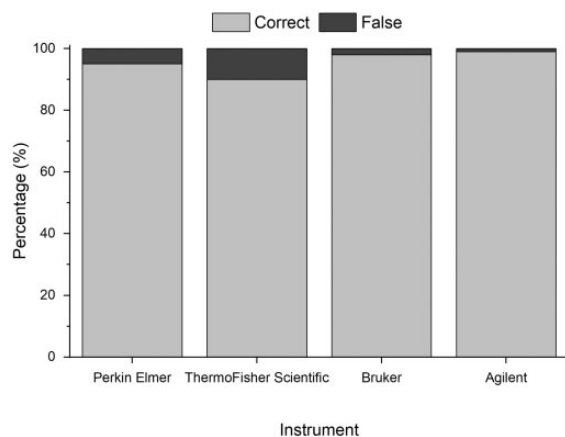
Figure 6. Assignment rates of correct and misidentified spectra for the different instruments based on manual reanalysis similar to Primpke et al. 21
