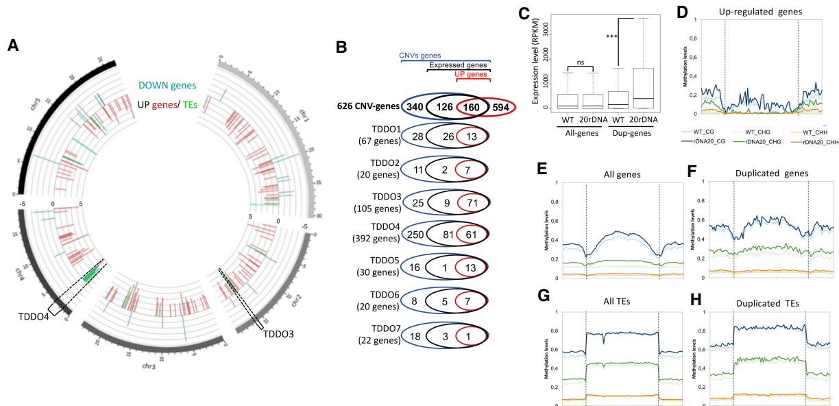
Figure 5. Impact of TDDO on global gene expression and cytosine methylation in L6F6. (A) Representation of the chromosomal position of genes (red bars) and TEs (green bars) of differentially accumulated transcripts in the 20rDNA L6F6 versus WT Col-0 with an adjusted P -value < 0.01 and a \log_2 (fold change) > 2. Data are displayed using Circos (Krzywinski et al. 2009). The brackets display the position of TDDO3 and TDDO4. (B) Venn diagrams representing the proportion of expressed genes (containing at least two reads/genes in wild-type) and up-regulated genes ( P -value < 0.01, FC > 2) among all the duplicated genes or in each TDDO in L6F6. (C) Dot plot revealing the relative expression of all genes or duplicated (DUP) genes in leaves of 3-wk-old plants in WT Col-0 or in 20rDNA L6F6. (***) P -value = 0.0005 was calculated using a Wilcoxon test. (D–H) Global DNA methylation analyses from genome-wide bisulfite sequencing experiments in WT Col-0 versus the 20rDNA L6F6. Global CG, CHG, and CHH methylation are shown for up-regulated genes with an adjusted P -value < 0.01 and a \log_2 (fold change) > 1.5 (D), all genes (E), duplicated genes (F), all TEs (G), and duplicated TEs (H).
