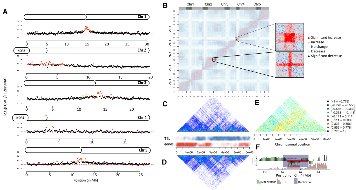
Figure 3. 3D genome organization in L6F6. (A) Chromosome plots displaying the relative enrichment of a given genomic segment with the nucleolus. The y-axis displays the fold change nucleolus enrichment between wild-type Col-0 and the 20rDNA L6F6. Each dot represents a 100-kb window. Nucleolus-enriched genomic regions above the threshold are red, and depleted regions are violet. (B) Coverage-normalized t -test difference matrix (50-kb bins). The color of each pixel of the matrix is defined by the result of a t -test using the triplicate contact frequencies from wild-type and 20rDNA coverage-normalized Hi-C samples. The two magnified areas correspond to the two regions displaying the highest level of contact frequency changes. (C,D) Non-normalized Hi-C snapshot showing the contact frequencies on the short arm of Chromosome 4 in wild-type Col-0 (C) versus the 20rDNA L6F6 (D). TEs and genes are annotated to illustrate the occurrence of euchromatin and heterochromatin, respectively. (E) Ratio between Hi-C contact frequencies from wild-type and 20rDNA L6F6. Negative ratios correspond to more contacts in the wild type, whereas positive ratios correspond to more contacts in the 20rDNA L6F6. (F) Eigenvector of the wild-type Col-0 Hi-C data set and annotation of the TDDO4 affecting the knob hk4s. Note the central duplication breakpoint exactly coincides with a change between LSD and a CSD.
