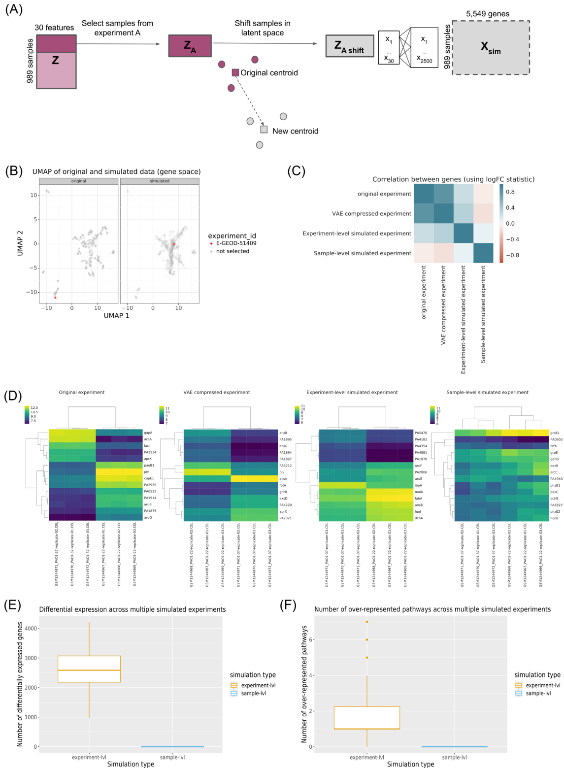
Figure 3: Simulating gene expression compendia by experiment. (A) Workflow to simulate gene expression per experiment. (B) UMAP projection of P. aeruginosa gene expression data highlighting a single experiment, E-GEOD-51409 (red), in the original dataset (left) and the simulated dataset (right), which was subsampled to 1,000 samples. (C) Correlation matrix showing the correlation between genes, based on their logFC, in the original experiment (E-GEOD-51409) vs VAE compressed experiment; original experiment vs simulated experiment using the original experiment as a template (experiment-level simulated); original vs random simulated (sample-level simulated) experiment. (D) Differential expression analysis of experiment E-GEOD-51409 (left), VAE-compressed experiment (middle-left); original vs random simulated (middle-right), and simulated experiment using the original experiment as a template (right). (E) Number of differentially expressed genes identified across 100 simulated experiments generated using experiment-level simulation and sample-level simulation. (F) Number of enriched pathways identified across 100 simulated experiments generated using experiment-level simulation and sample-level simulation. Circles denote outliers.logFC: log fold-change.
