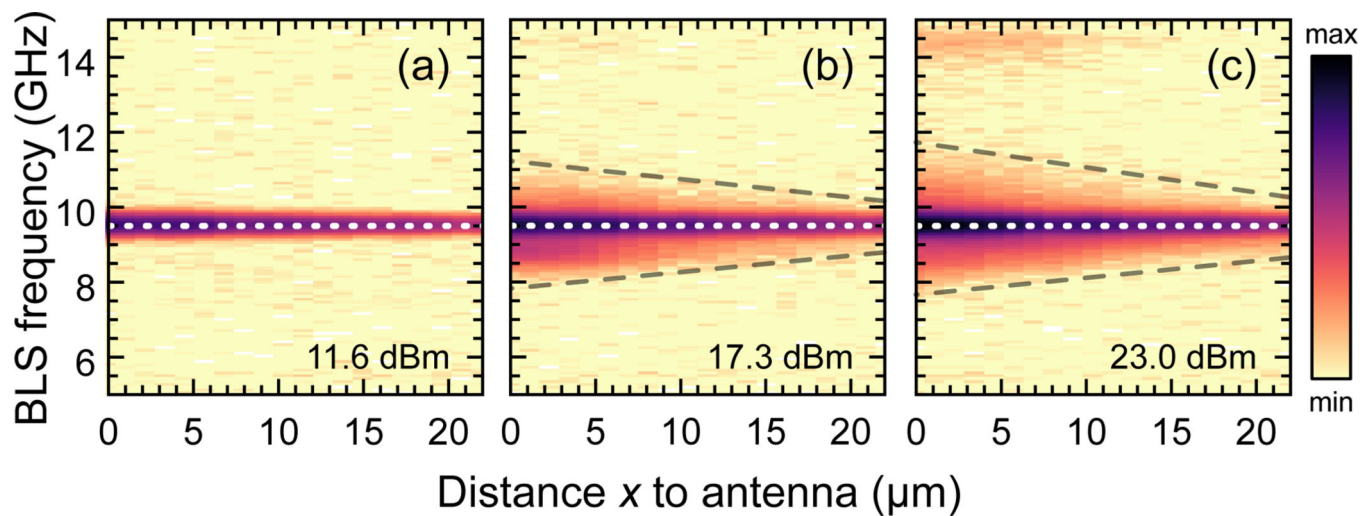
FIG. 3. \mu BLS spectra measured along the waveguide for different excitation powers at a fixed excitation frequency f_{\text{rf}} = 9.5 GHz (white dotted line). The grey dashed lines mark the distribution of magnons that are parametrically excited by four-magnon scattering.
