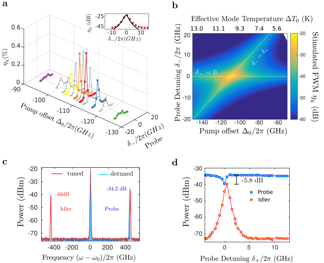
Fig. 2. Stimulated Four Wave Mixing
