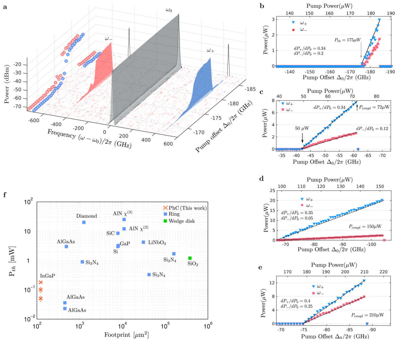
Fig. 3. Parametric Oscillation
