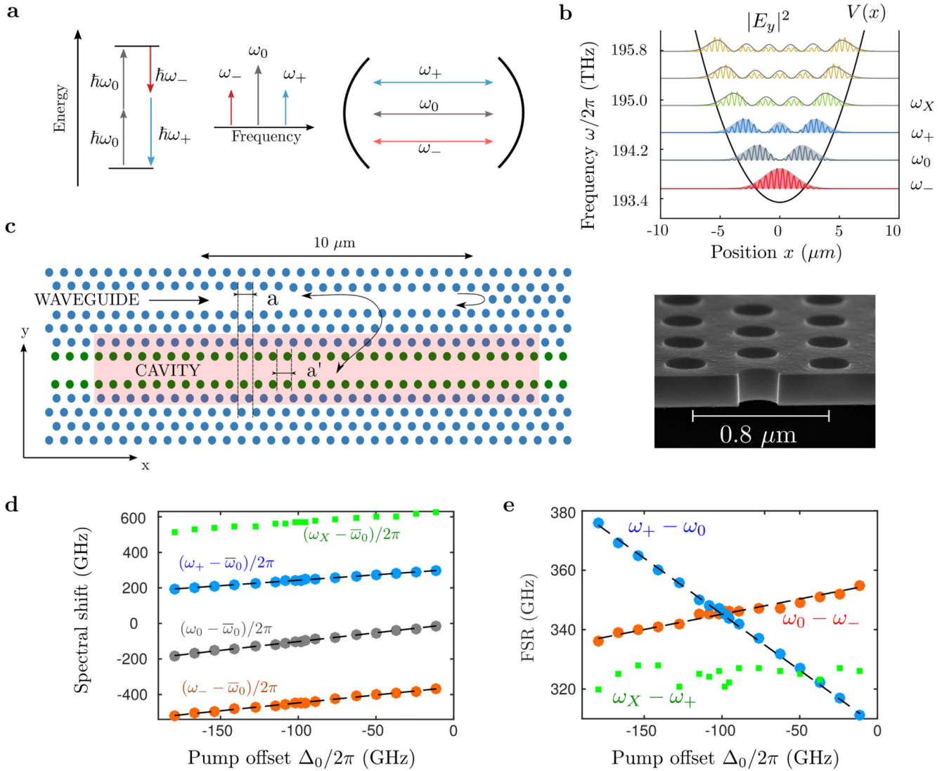
Fig. 1. Triply resonant PhC cavity
