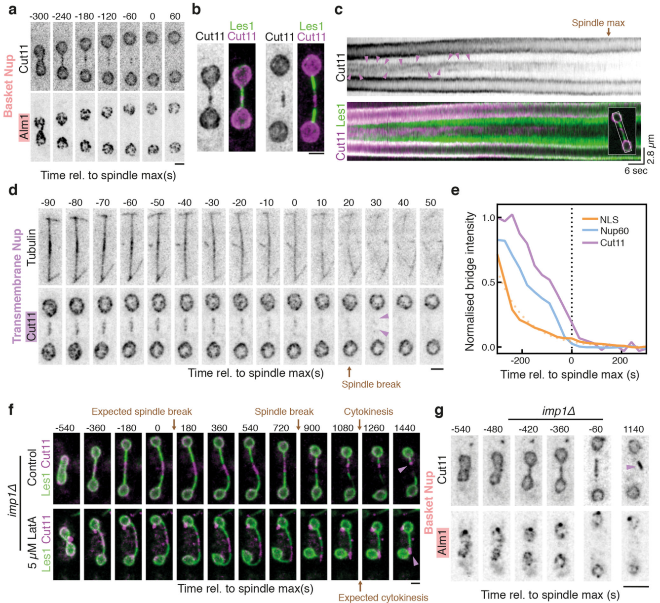
Figure 3. Les1-restricted stepwise NPC disassembly drives local NEB
